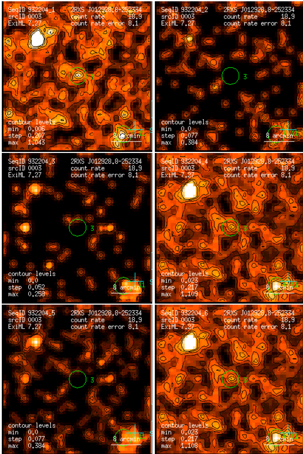
Figure 3: RASS 932204: detection 0003: band rate images, Gaussian filter: (1) PSPC channels 11 – 41, (2) 52 – 90, (3) 91 – 201, (4) 11 – 235, (5) 52 – 201, (6) 11 – 201. Broad band rates in counts/ks. Band rate contour levels in counts/ks/arcmin 2 .
