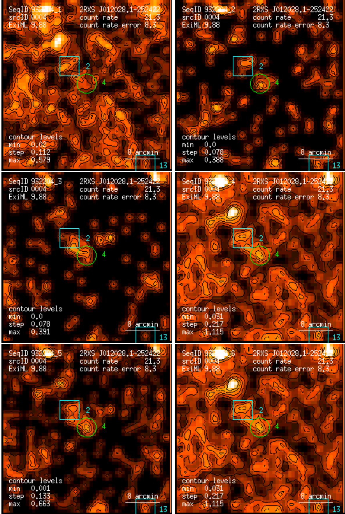
Figure 4: RASS 932204: detection 0004: band rate images, Gaussian filter: (1) PSPC channels 11 – 41, (2) 52 – 90, (3) 91 – 201, (4) 11 – 235, (5) 52 – 201, (6) 11 – 201. Broad band rates in counts/ks. Band rate contour levels in counts/ks/arcmin 2 .
