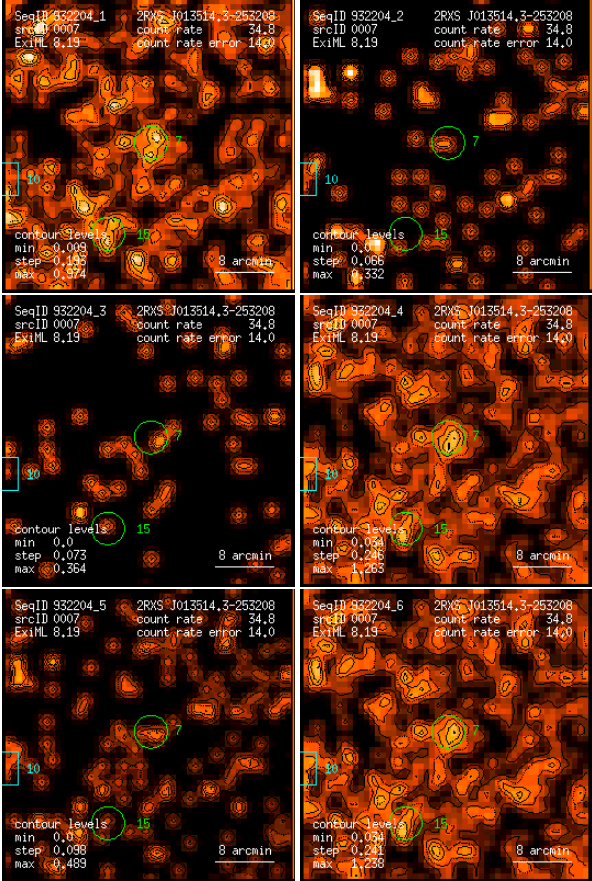
Figure 7: RASS 932204: detection 0007: band rate images, Gaussian filter: (1) PSPC channels 11 – 41, (2) 52 – 90, (3) 91 – 201, (4) 11 – 235, (5) 52 – 201, (6) 11 – 201. Broad band rates in counts/ks. Band rate contour levels in counts/ks/arcmin 2 .
