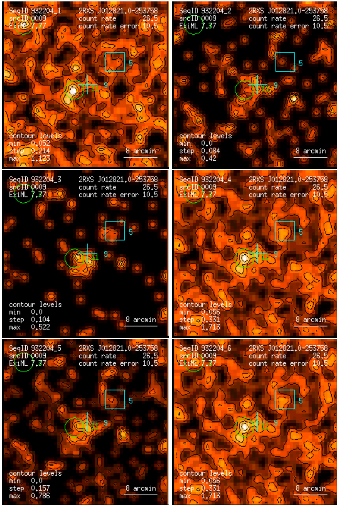
Figure 9: RASS 932204: detection 0009: band rate images, Gaussian filter: (1) PSPC channels 11 – 41, (2) 52 – 90, (3) 91 – 201, (4) 11 – 235, (5) 52 – 201, (6) 11 – 201. Broad band rates in counts/ks. Band rate contour levels in counts/ks/arcmin 2 .
