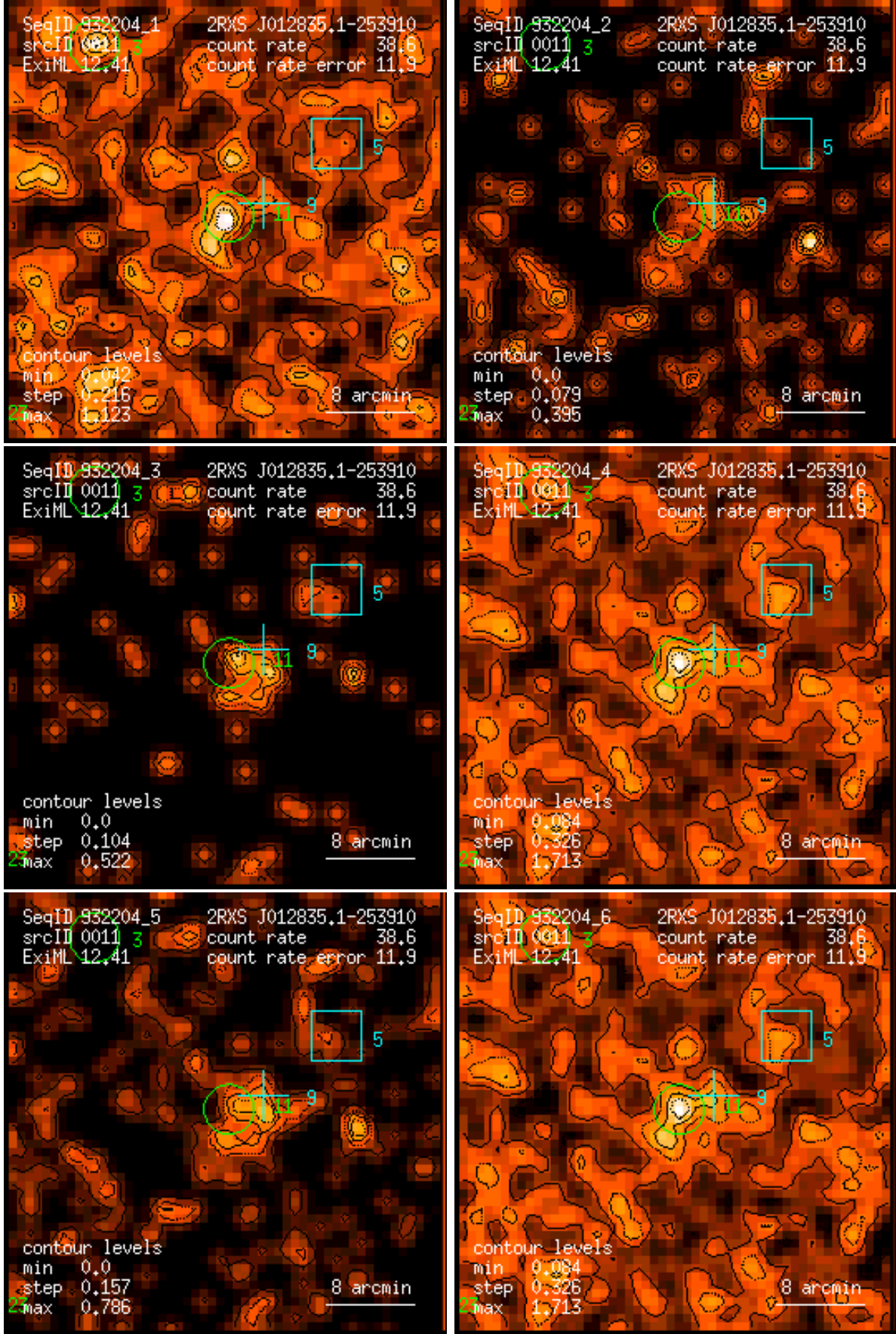
Figure 11: RASS 932204: detection 0011: band rate images, Gaussian filter: (1) PSPC channels 11 – 41, (2) 52 – 90, (3) 91 – 201, (4) 11 – 235, (5) 52 – 201, (6) 11 – 201. Broad band rates in counts/ks. Band rate contour levels in counts/ks/arcmin 2 .
