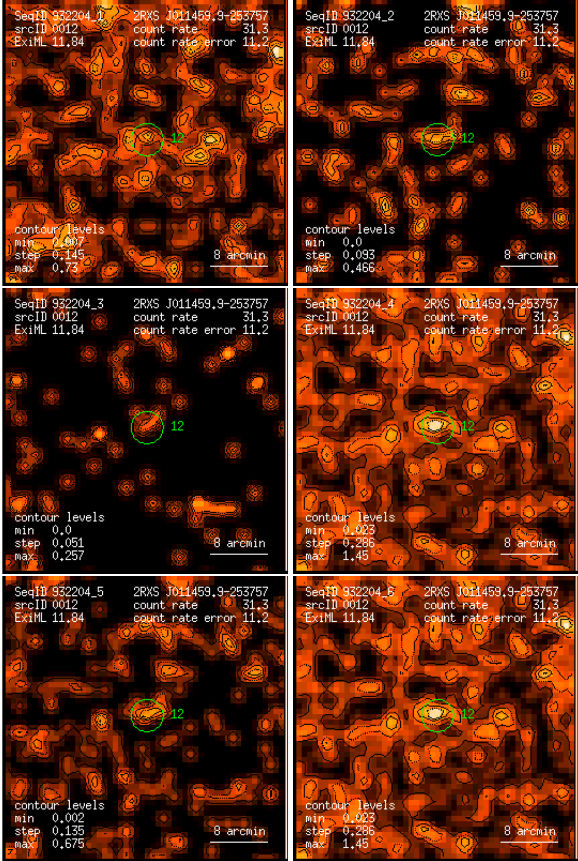
Figure 12: RASS 932204: detection 0012: band rate images, Gaussian filter: (1) PSPC channels 11 – 41, (2) 52 – 90, (3) 91 – 201, (4) 11 – 235, (5) 52 – 201, (6) 11 – 201. Broad band rates in counts/ks. Band rate contour levels in counts/ks/arcmin 2 .
