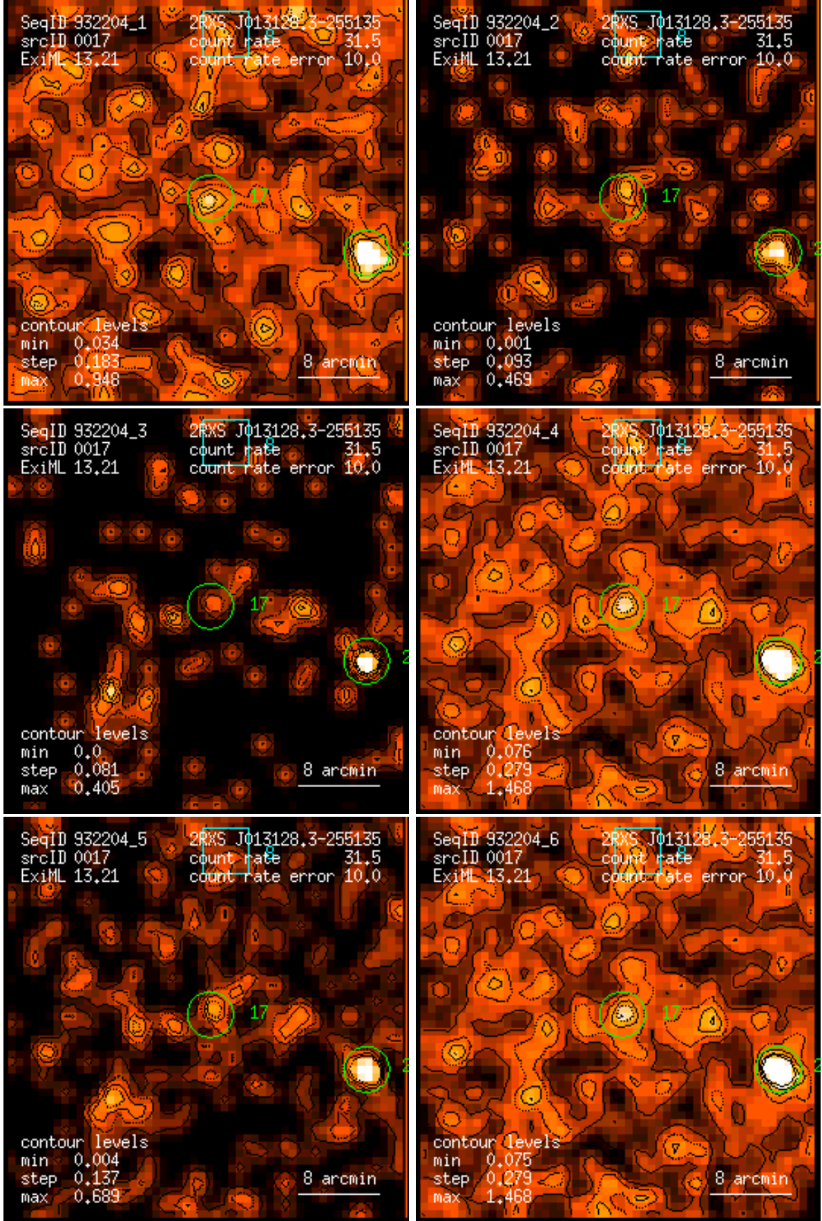
Figure 17: RASS 932204: detection 0017: band rate images, Gaussian filter: (1) PSPC channels 11 – 41, (2) 52 – 90, (3) 91 – 201, (4) 11 – 235, (5) 52 – 201, (6) 11 – 201. Broad band rates in counts/ks. Band rate contour levels in counts/ks/arcmin 2 .
