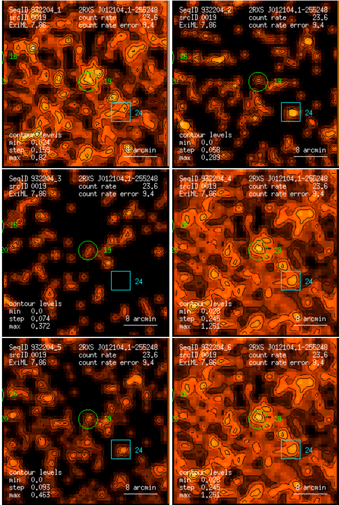
Figure 19: RASS 932204: detection 0019: band rate images, Gaussian filter: (1) PSPC channels 11 – 41, (2) 52 – 90, (3) 91 – 201, (4) 11 – 235, (5) 52 – 201, (6) 11 – 201. Broad band rates in counts/ks. Band rate contour levels in counts/ks/arcmin 2 .
