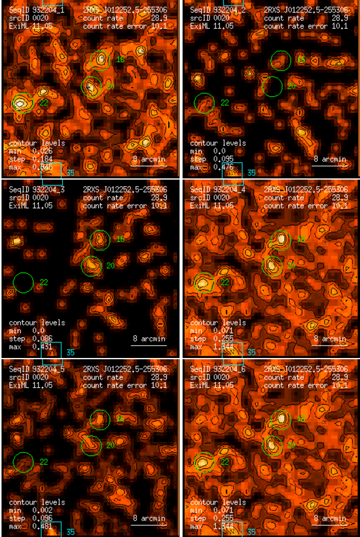
Figure 20: RASS 932204: detection 0020: band rate images, Gaussian filter: (1) PSPC channels 11 – 41, (2) 52 – 90, (3) 91 – 201, (4) 11 – 235, (5) 52 – 201, (6) 11 – 201. Broad band rates in counts/ks. Band rate contour levels in counts/ks/arcmin 2 .
