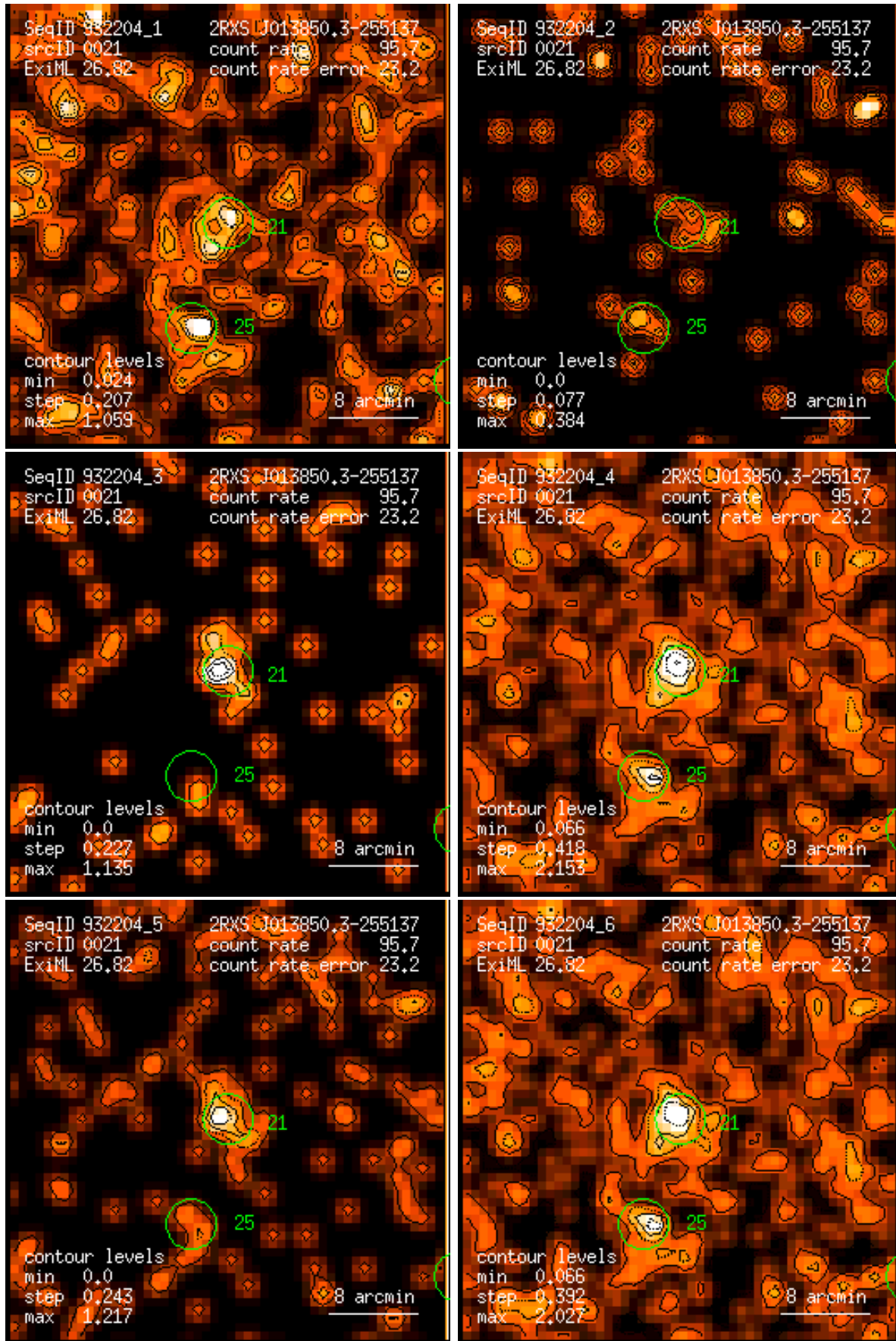
Figure 21: RASS 932204: detection 0021: band rate images, Gaussian filter: (1) PSPC channels 11 – 41, (2) 52 – 90, (3) 91 – 201, (4) 11 – 235, (5) 52 – 201, (6) 11 – 201. Broad band rates in counts/ks. Band rate contour levels in counts/ks/arcmin 2 .
