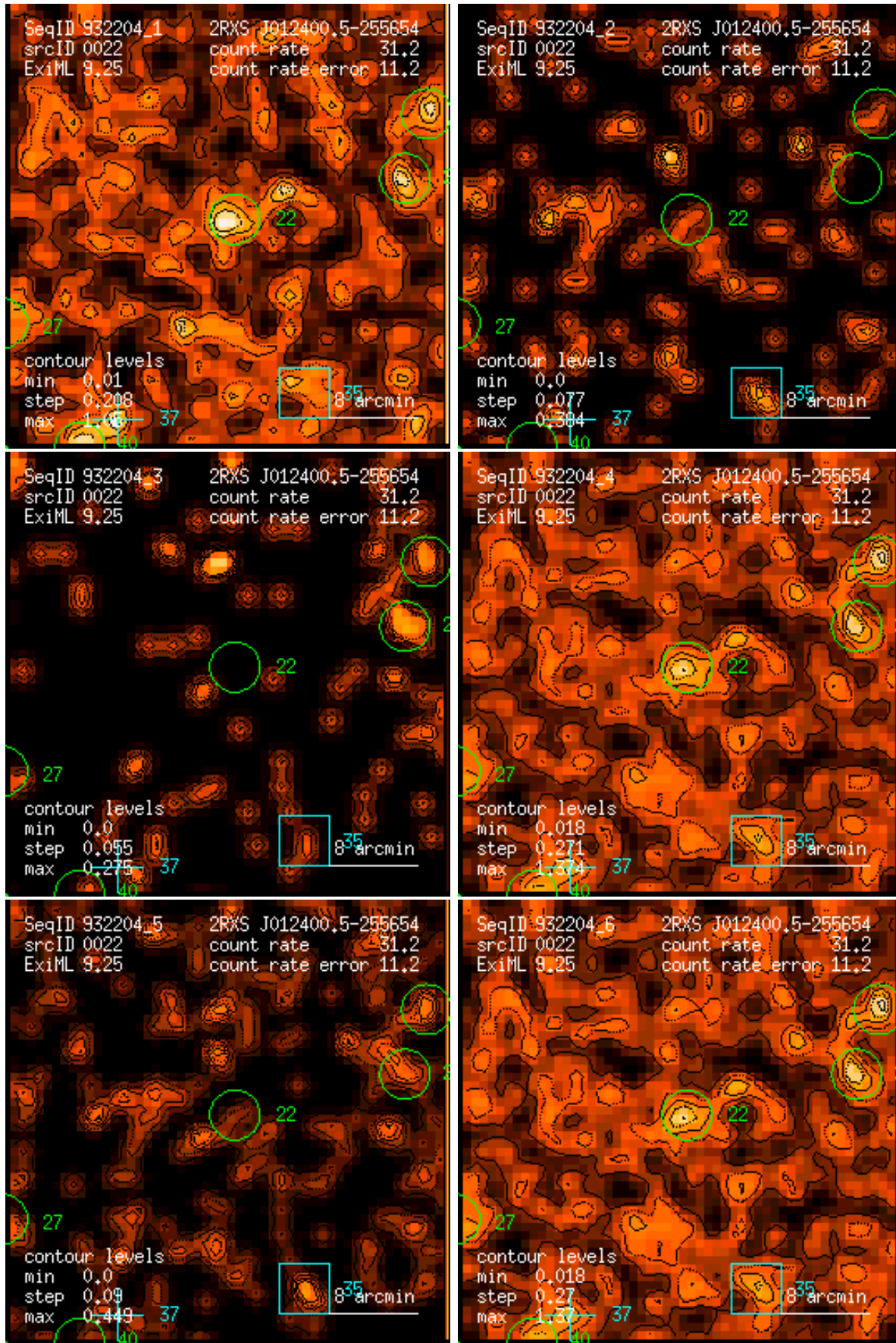
Figure 22: RASS 932204: detection 0022: band rate images, Gaussian filter: (1) PSPC channels 11 – 41, (2) 52 – 90, (3) 91 – 201, (4) 11 – 235, (5) 52 – 201, (6) 11 – 201. Broad band rates in counts/ks. Band rate contour levels in counts/ks/arcmin 2 .
