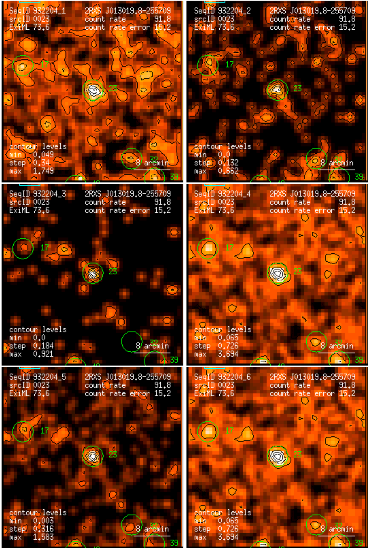
Figure 23: RASS 932204: detection 0023: band rate images, Gaussian filter: (1) PSPC channels 11 – 41, (2) 52 – 90, (3) 91 – 201, (4) 11 – 235, (5) 52 – 201, (6) 11 – 201. Broad band rates in counts/ks. Band rate contour levels in counts/ks/arcmin 2 .
