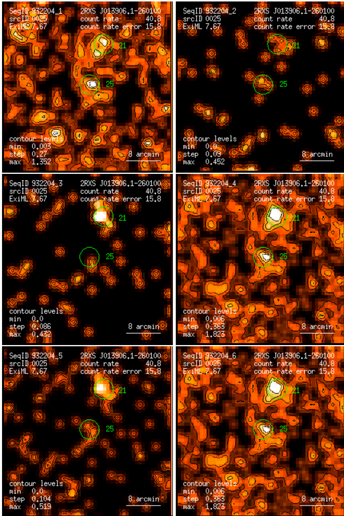
Figure 25: RASS 932204: detection 0025: band rate images, Gaussian filter: (1) PSPC channels 11 – 41, (2) 52 – 90, (3) 91 – 201, (4) 11 – 235, (5) 52 – 201, (6) 11 – 201. Broad band rates in counts/ks. Band rate contour levels in counts/ks/arcmin 2 .
