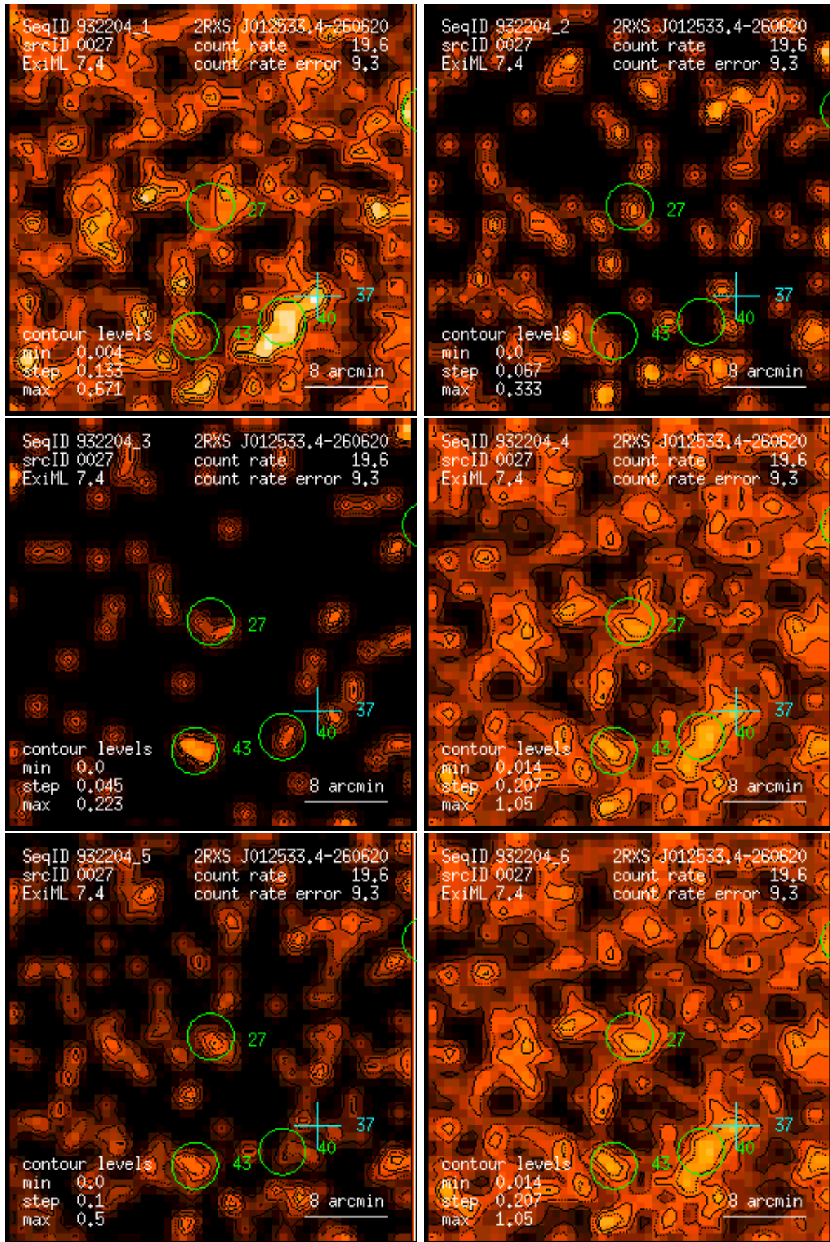
Figure 27: RASS 932204: detection 0027: band rate images, Gaussian filter: (1) PSPC channels 11 – 41, (2) 52 – 90, (3) 91 – 201, (4) 11 – 235, (5) 52 – 201, (6) 11 – 201. Broad band rates in counts/ks. Band rate contour levels in counts/ks/arcmin 2 .
