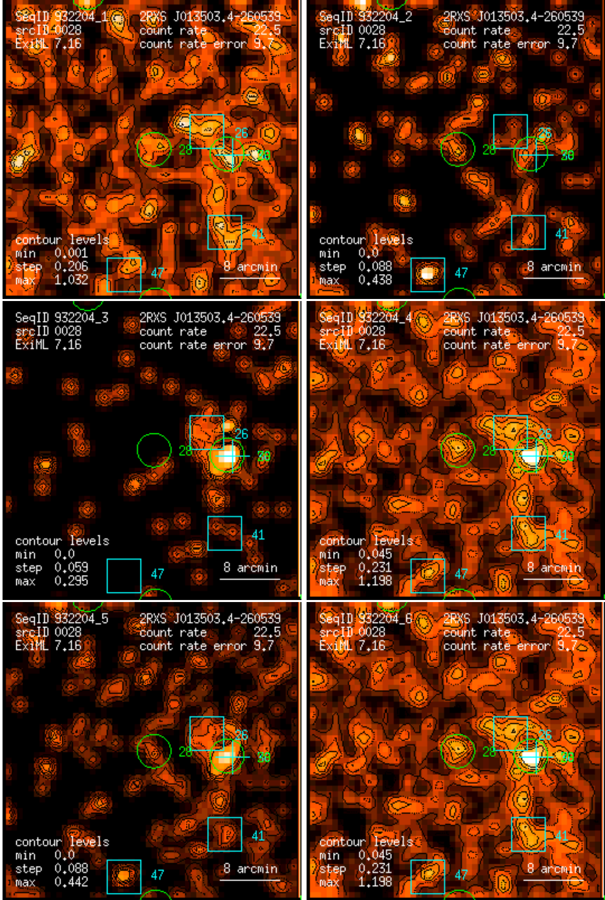
Figure 28: RASS 932204: detection 0028: band rate images, Gaussian filter: (1) PSPC channels 11 – 41, (2) 52 – 90, (3) 91 – 201, (4) 11 – 235, (5) 52 – 201, (6) 11 – 201. Broad band rates in counts/ks. Band rate contour levels in counts/ks/arcmin 2 .
