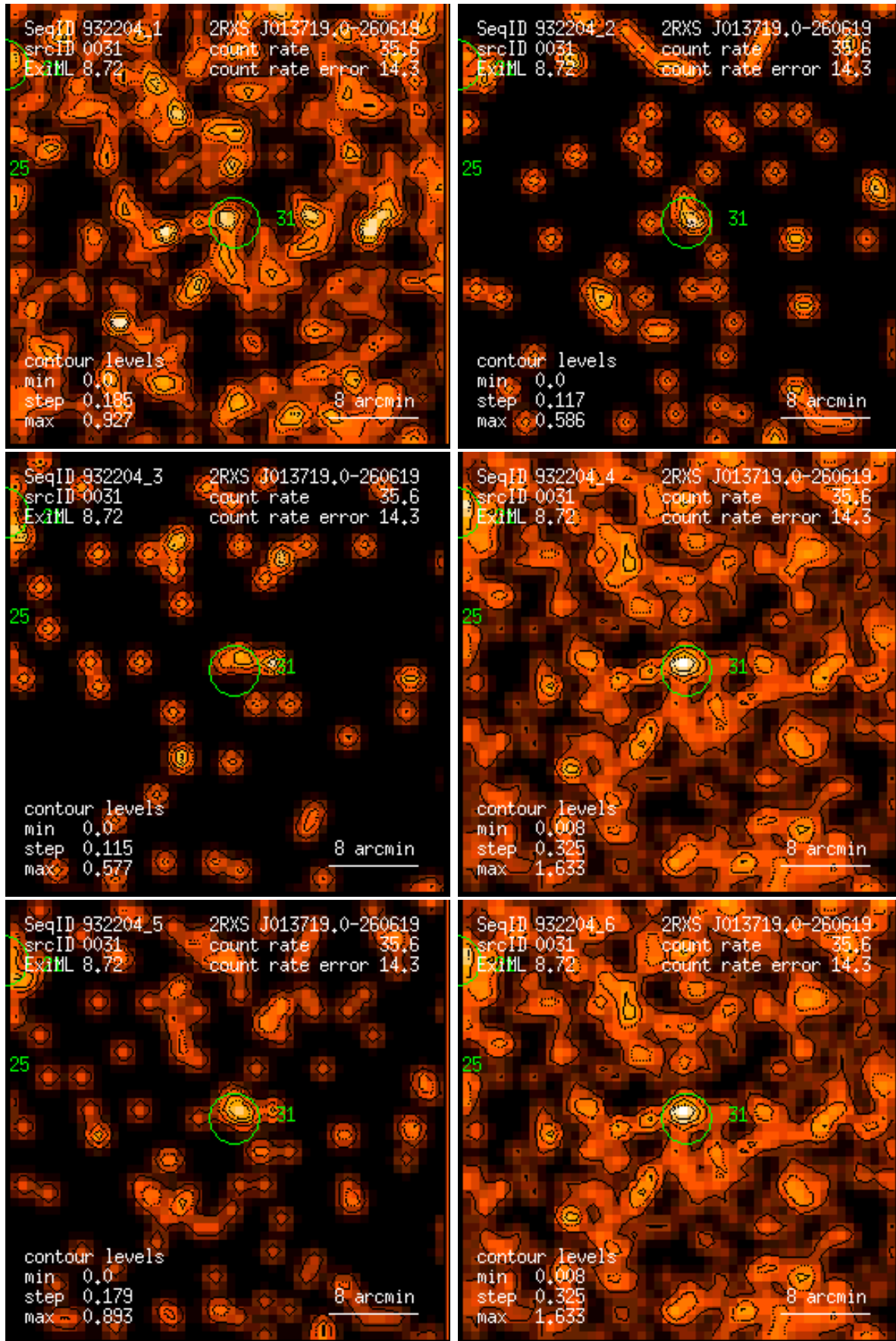
Figure 31: RASS 932204: detection 0031: band rate images, Gaussian filter: (1) PSPC channels 11 – 41, (2) 52 – 90, (3) 91 – 201, (4) 11 – 235, (5) 52 – 201, (6) 11 – 201. Broad band rates in counts/ks. Band rate contour levels in counts/ks/arcmin 2 .
