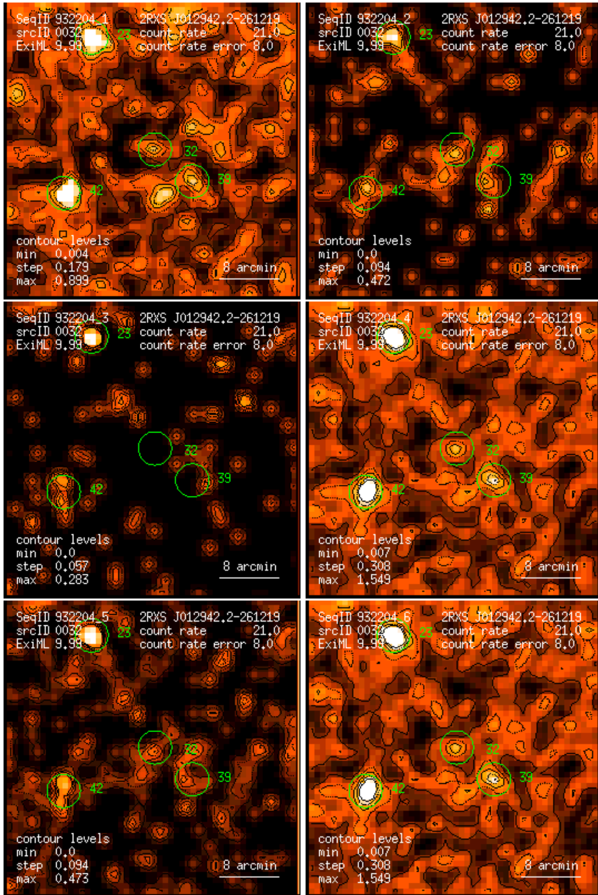
Figure 32: RASS 932204: detection 0032: band rate images, Gaussian filter: (1) PSPC channels 11 – 41, (2) 52 – 90, (3) 91 – 201, (4) 11 – 235, (5) 52 – 201, (6) 11 – 201. Broad band rates in counts/ks. Band rate contour levels in counts/ks/arcmin 2 .
