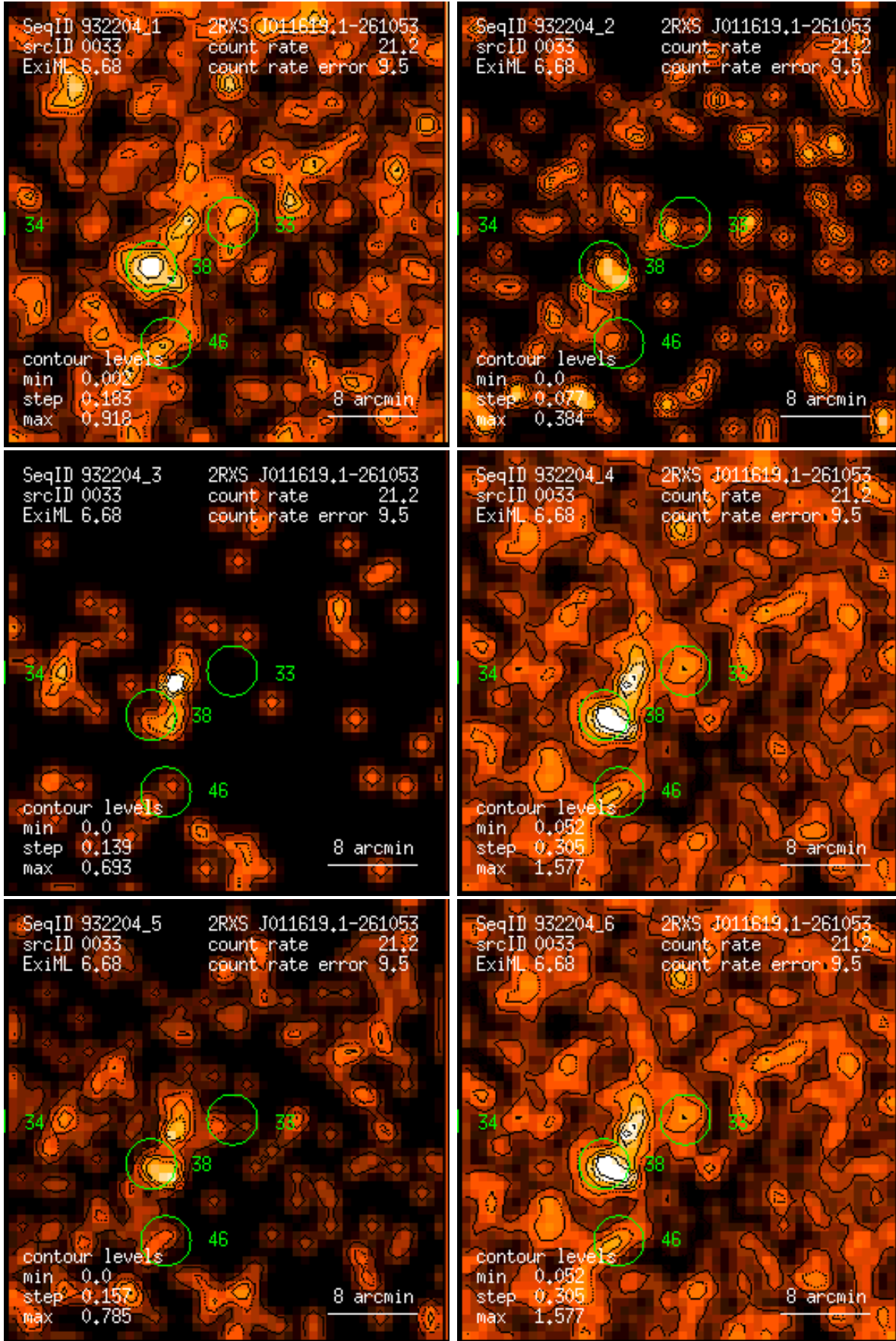
Figure 33: RASS 932204: detection 0033: band rate images, Gaussian filter: (1) PSPC channels 11 – 41, (2) 52 – 90, (3) 91 – 201, (4) 11 – 235, (5) 52 – 201, (6) 11 – 201. Broad band rates in counts/ks. Band rate contour levels in counts/ks/arcmin 2 .
