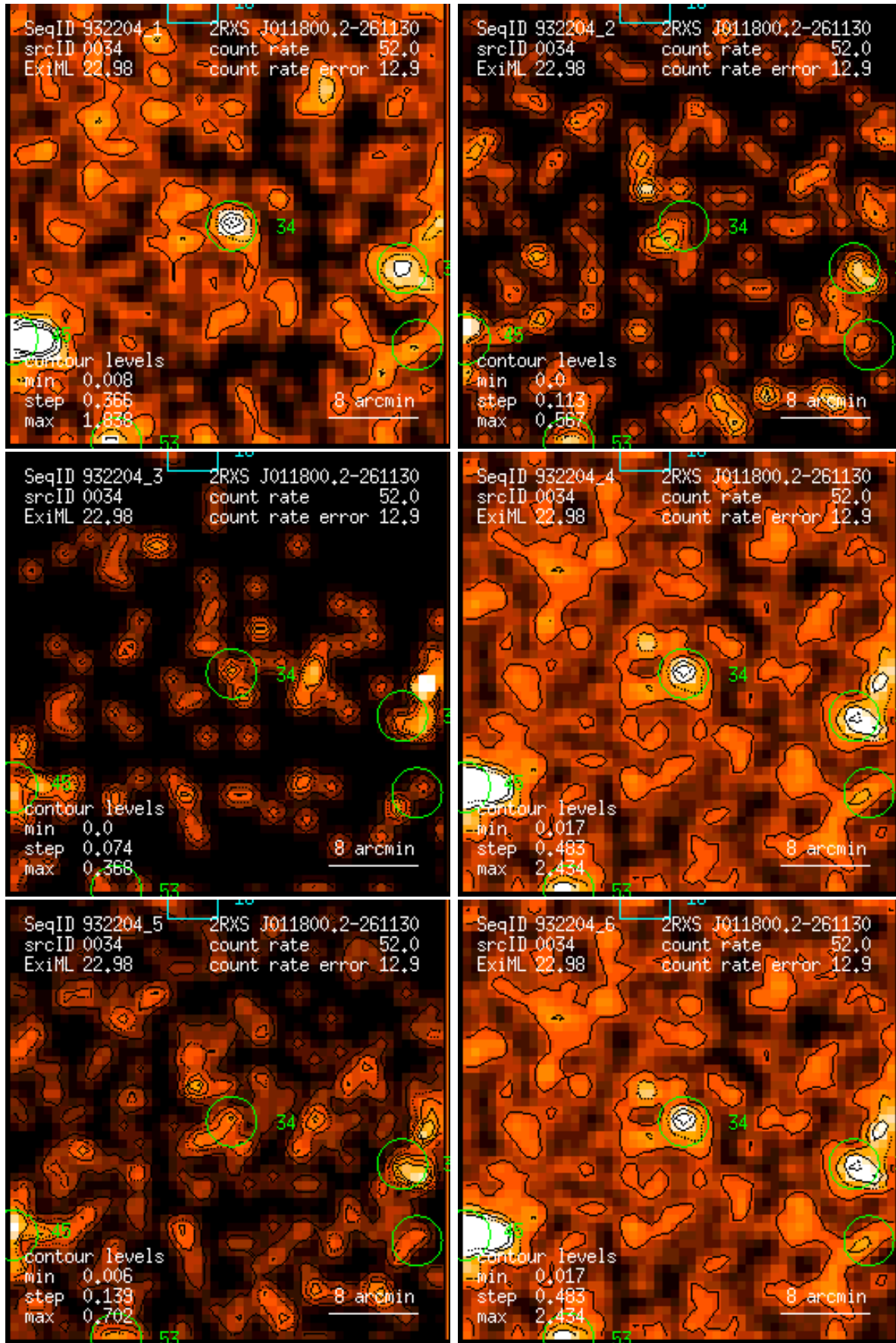
Figure 34: RASS 932204: detection 0034: band rate images, Gaussian filter: (1) PSPC channels 11 – 41, (2) 52 – 90, (3) 91 – 201, (4) 11 – 235, (5) 52 – 201, (6) 11 – 201. Broad band rates in counts/ks. Band rate contour levels in counts/ks/arcmin 2 .
