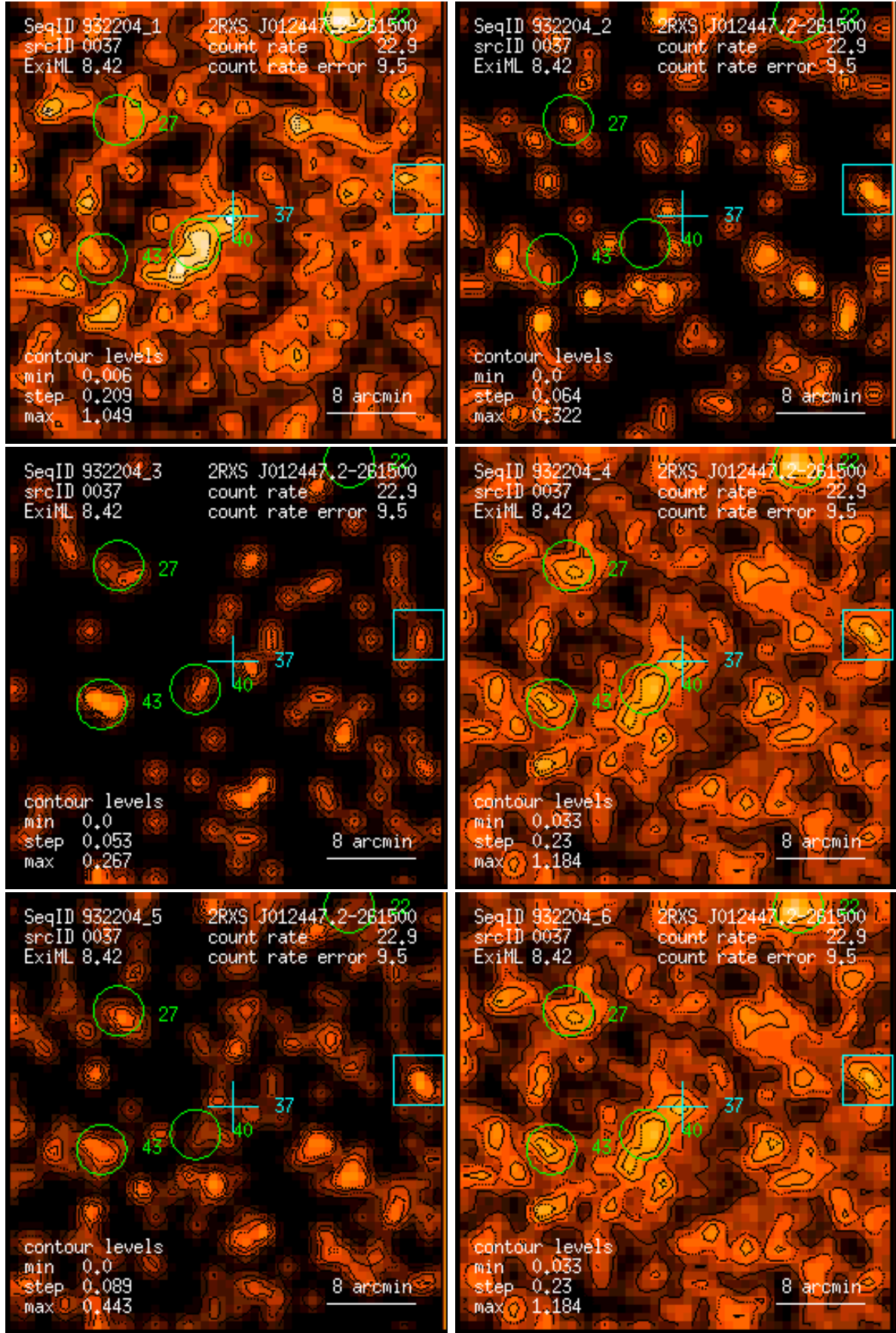
Figure 37: RASS 932204: detection 0037: band rate images, Gaussian filter: (1) PSPC channels 11 – 41, (2) 52 – 90, (3) 91 – 201, (4) 11 – 235, (5) 52 – 201, (6) 11 – 201. Broad band rates in counts/ks. Band rate contour levels in counts/ks/arcmin 2 .
