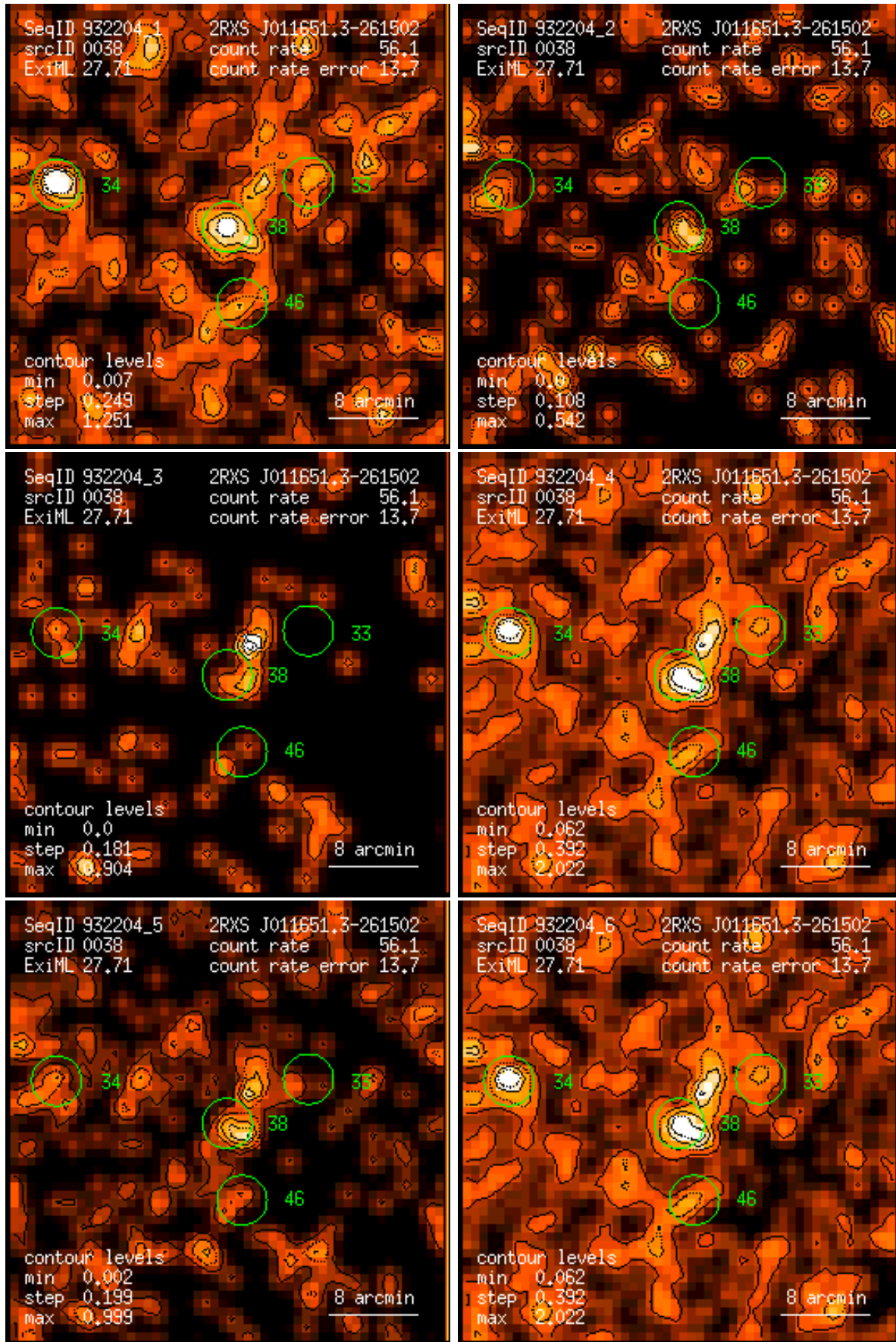
Figure 38: RASS 932204: detection 0038: band rate images, Gaussian filter: (1) PSPC channels 11 – 41, (2) 52 – 90, (3) 91 – 201, (4) 11 – 235, (5) 52 – 201, (6) 11 – 201. Broad band rates in counts/ks. Band rate contour levels in counts/ks/arcmin 2 .
