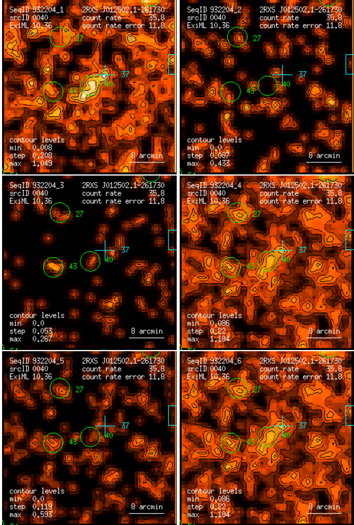
Figure 40: RASS 932204: detection 0040: band rate images, Gaussian filter: (1) PSPC channels 11 – 41, (2) 52 – 90, (3) 91 – 201, (4) 11 – 235, (5) 52 – 201, (6) 11 – 201. Broad band rates in counts/ks. Band rate contour levels in counts/ks/arcmin 2 .
