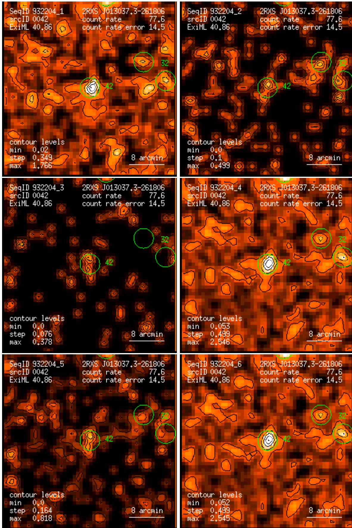
Figure 42: RASS 932204: detection 0042: band rate images, Gaussian filter: (1) PSPC channels 11 – 41, (2) 52 – 90, (3) 91 – 201, (4) 11 – 235, (5) 52 – 201, (6) 11 – 201. Broad band rates in counts/ks. Band rate contour levels in counts/ks/arcmin 2 .
