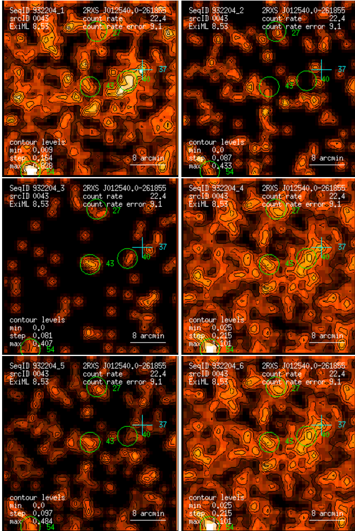
Figure 43: RASS 932204: detection 0043: band rate images, Gaussian filter: (1) PSPC channels 11 – 41, (2) 52 – 90, (3) 91 – 201, (4) 11 – 235, (5) 52 – 201, (6) 11 – 201. Broad band rates in counts/ks. Band rate contour levels in counts/ks/arcmin 2 .
