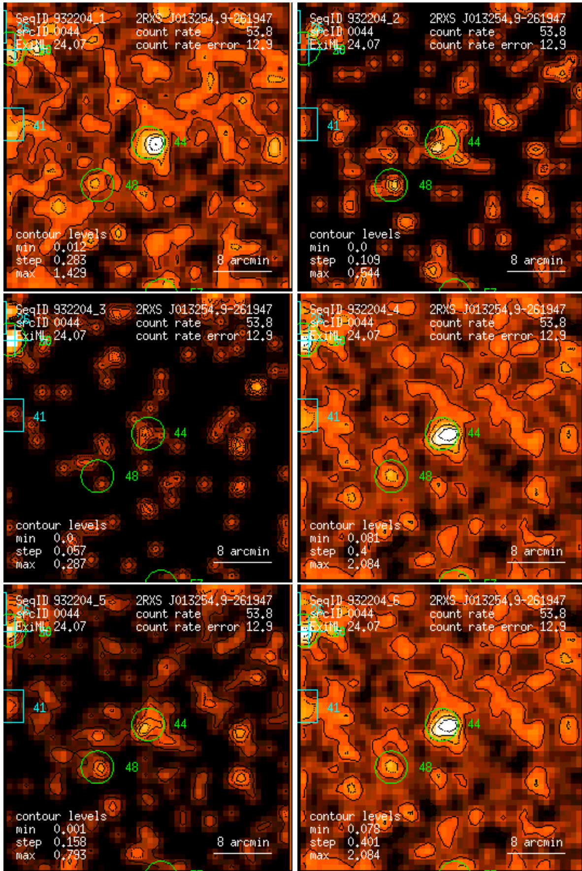
Figure 44: RASS 932204: detection 0044: band rate images, Gaussian filter: (1) PSPC channels 11 – 41, (2) 52 – 90, (3) 91 – 201, (4) 11 – 235, (5) 52 – 201, (6) 11 – 201. Broad band rates in counts/ks. Band rate contour levels in counts/ks/arcmin 2 .
