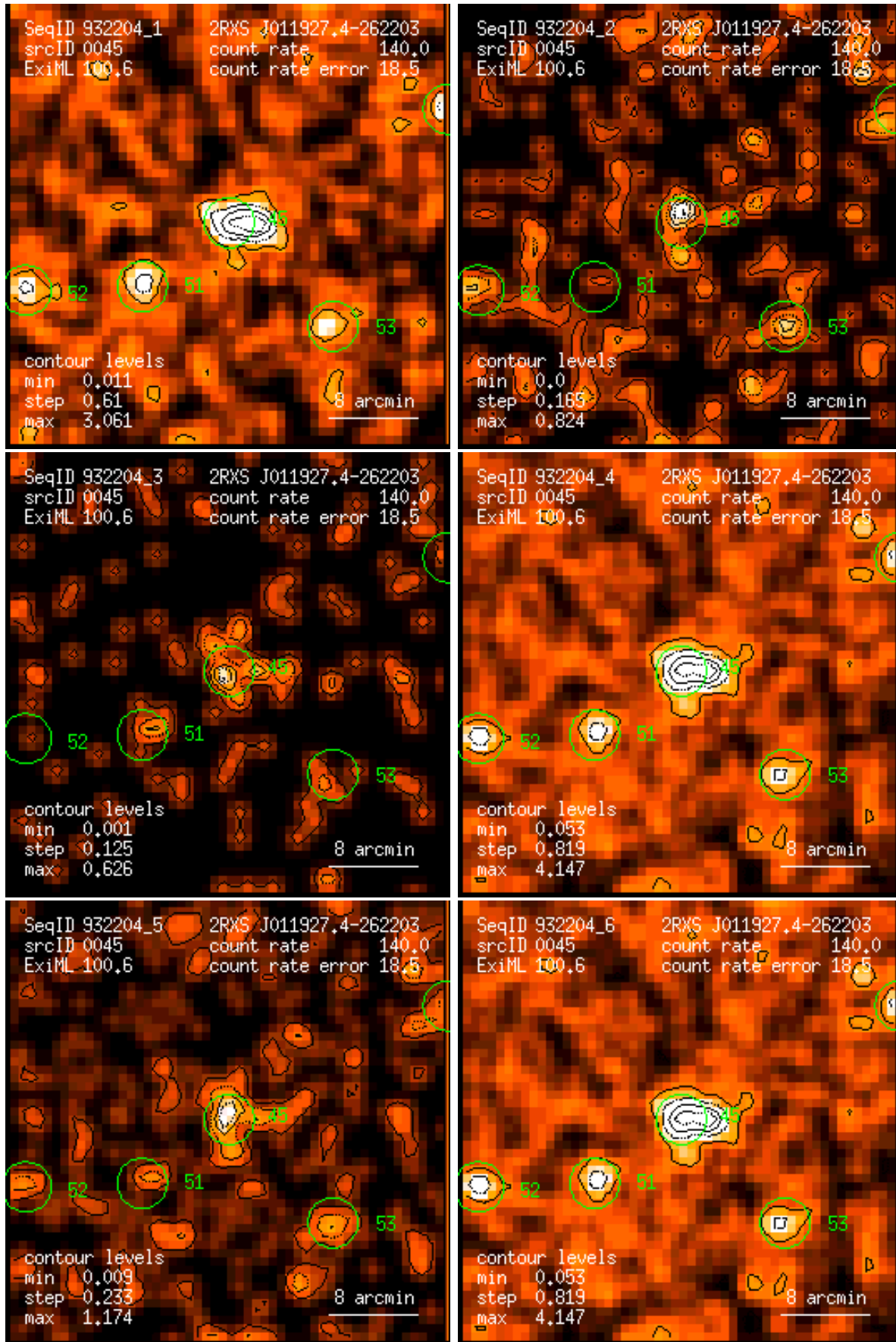
Figure 45: RASS 932204: detection 0045: band rate images, Gaussian filter: (1) PSPC channels 11 – 41, (2) 52 – 90, (3) 91 – 201, (4) 11 – 235, (5) 52 – 201, (6) 11 – 201. Broad band rates in counts/ks. Band rate contour levels in counts/ks/arcmin 2 .
