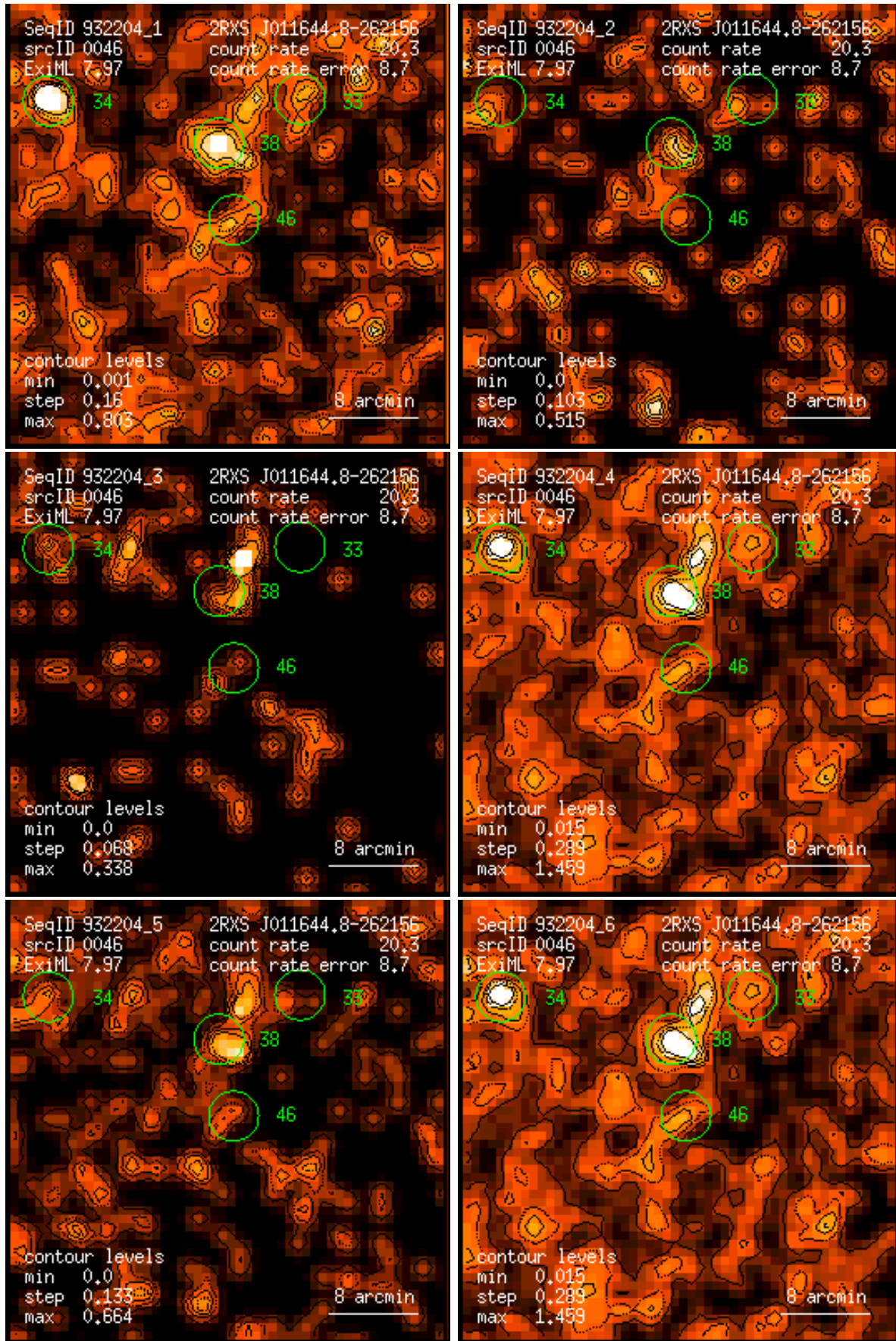
Figure 46: RASS 932204: detection 0046: band rate images, Gaussian filter: (1) PSPC channels 11 – 41, (2) 52 – 90, (3) 91 – 201, (4) 11 – 235, (5) 52 – 201, (6) 11 – 201. Broad band rates in counts/ks. Band rate contour levels in counts/ks/arcmin 2 .
