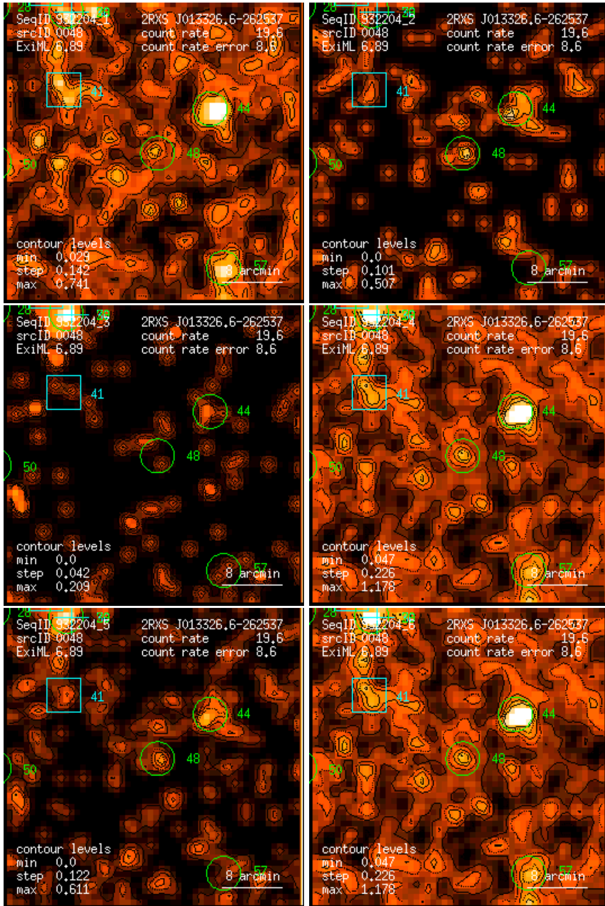
Figure 48: RASS 932204: detection 0048: band rate images, Gaussian filter: (1) PSPC channels 11 – 41, (2) 52 – 90, (3) 91 – 201, (4) 11 – 235, (5) 52 – 201, (6) 11 – 201. Broad band rates in counts/ks. Band rate contour levels in counts/ks/arcmin 2 .
