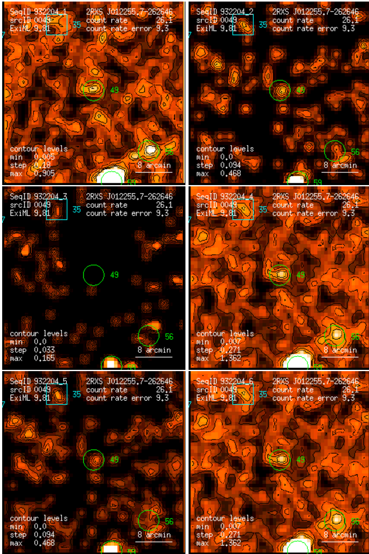
Figure 49: RASS 932204: detection 0049: band rate images, Gaussian filter: (1) PSPC channels 11 – 41, (2) 52 – 90, (3) 91 – 201, (4) 11 – 235, (5) 52 – 201, (6) 11 – 201. Broad band rates in counts/ks. Band rate contour levels in counts/ks/arcmin 2 .
