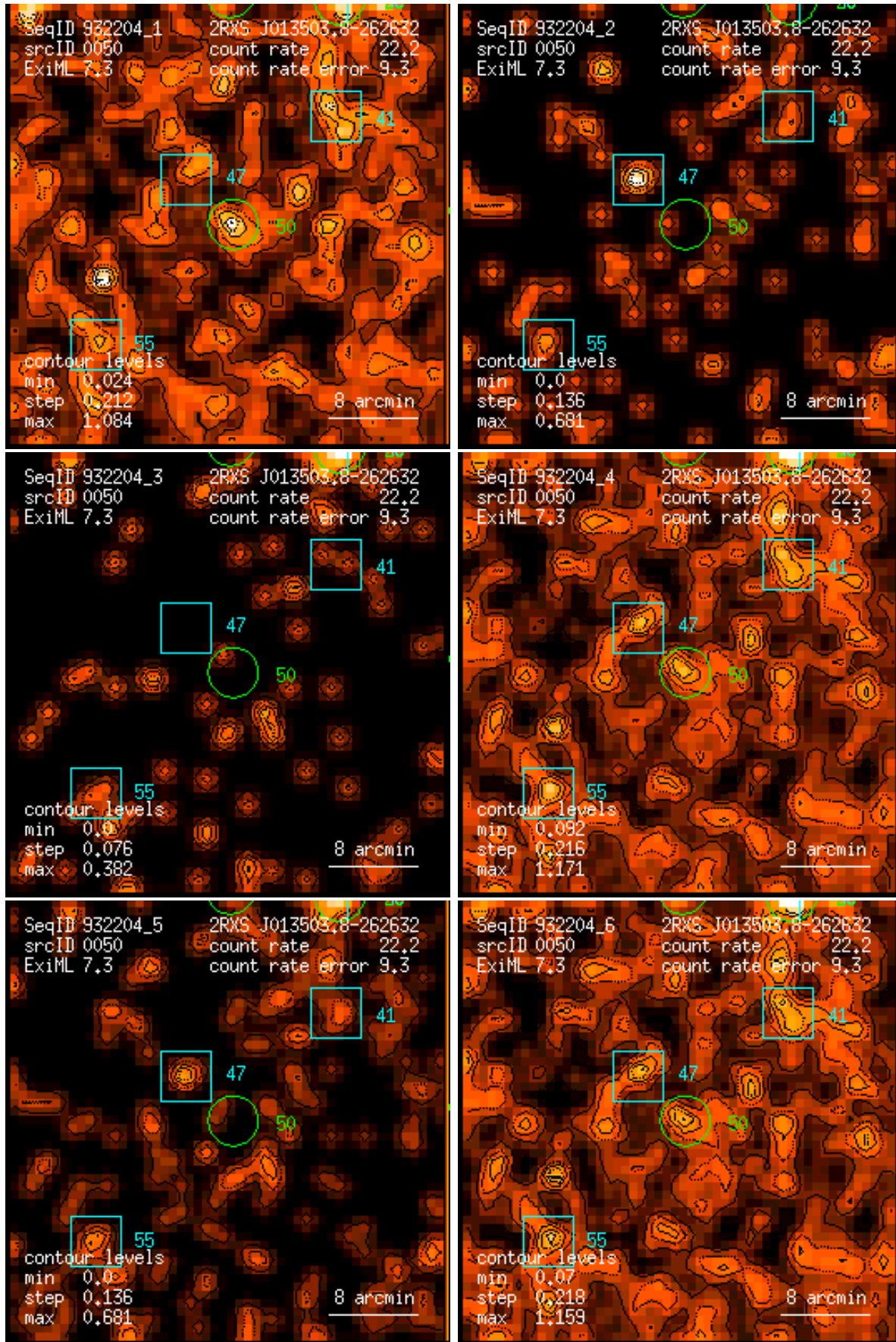
Figure 50: RASS 932204: detection 0050: band rate images, Gaussian filter: (1) PSPC channels 11 – 41, (2) 52 – 90, (3) 91 – 201, (4) 11 – 235, (5) 52 – 201, (6) 11 – 201. Broad band rates in counts/ks. Band rate contour levels in counts/ks/arcmin 2 .
