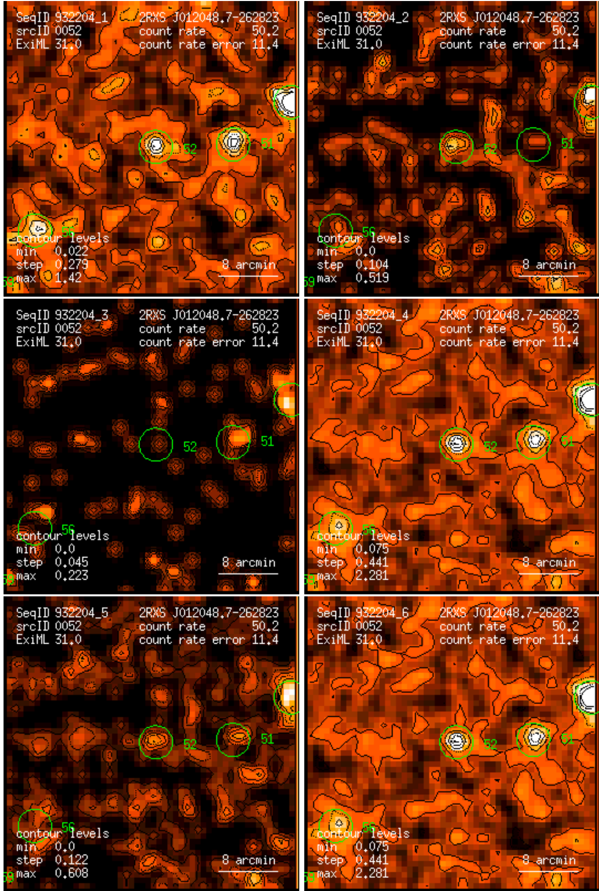
Figure 52: RASS 932204: detection 0052: band rate images, Gaussian filter: (1) PSPC channels 11 – 41, (2) 52 – 90, (3) 91 – 201, (4) 11 – 235, (5) 52 – 201, (6) 11 – 201. Broad band rates in counts/ks. Band rate contour levels in counts/ks/arcmin 2 .
