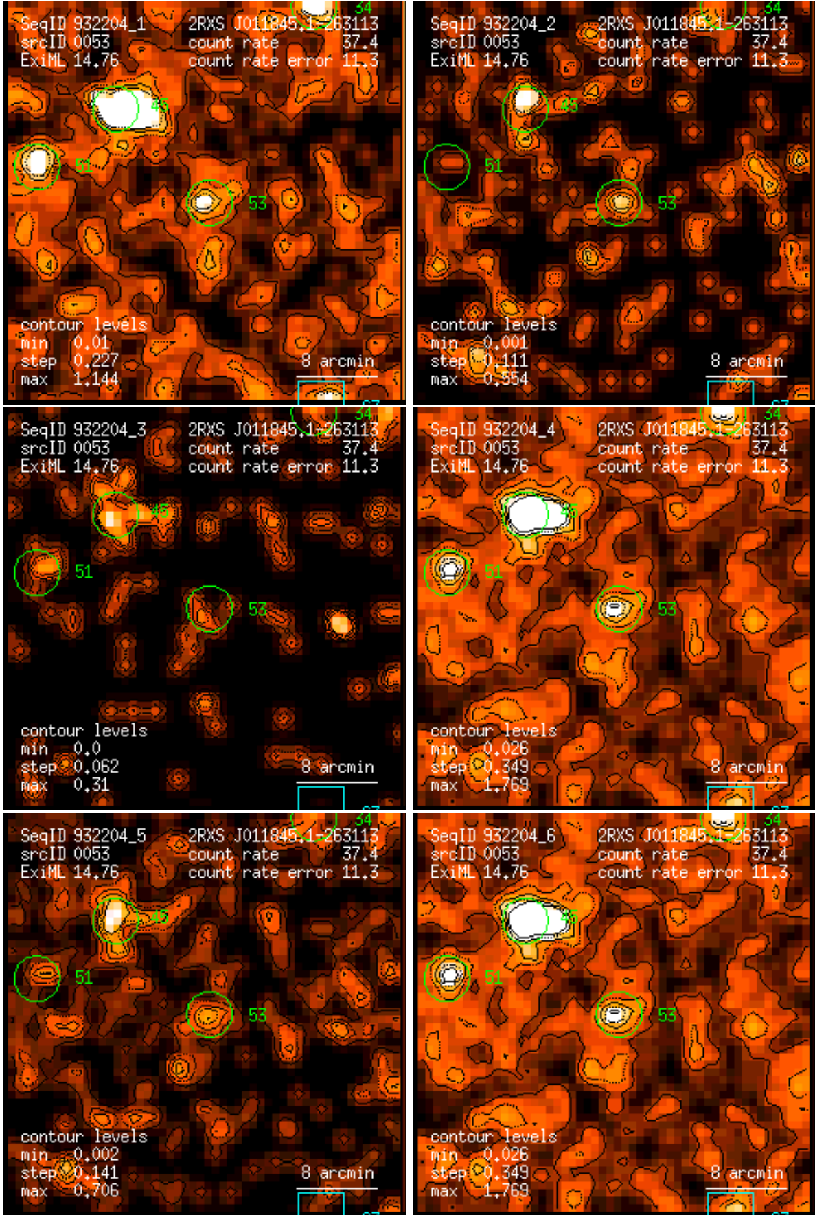
Figure 53: RASS 932204: detection 0053: band rate images, Gaussian filter: (1) PSPC channels 11 – 41, (2) 52 – 90, (3) 91 – 201, (4) 11 – 235, (5) 52 – 201, (6) 11 – 201. Broad band rates in counts/ks. Band rate contour levels in counts/ks/arcmin 2 .
