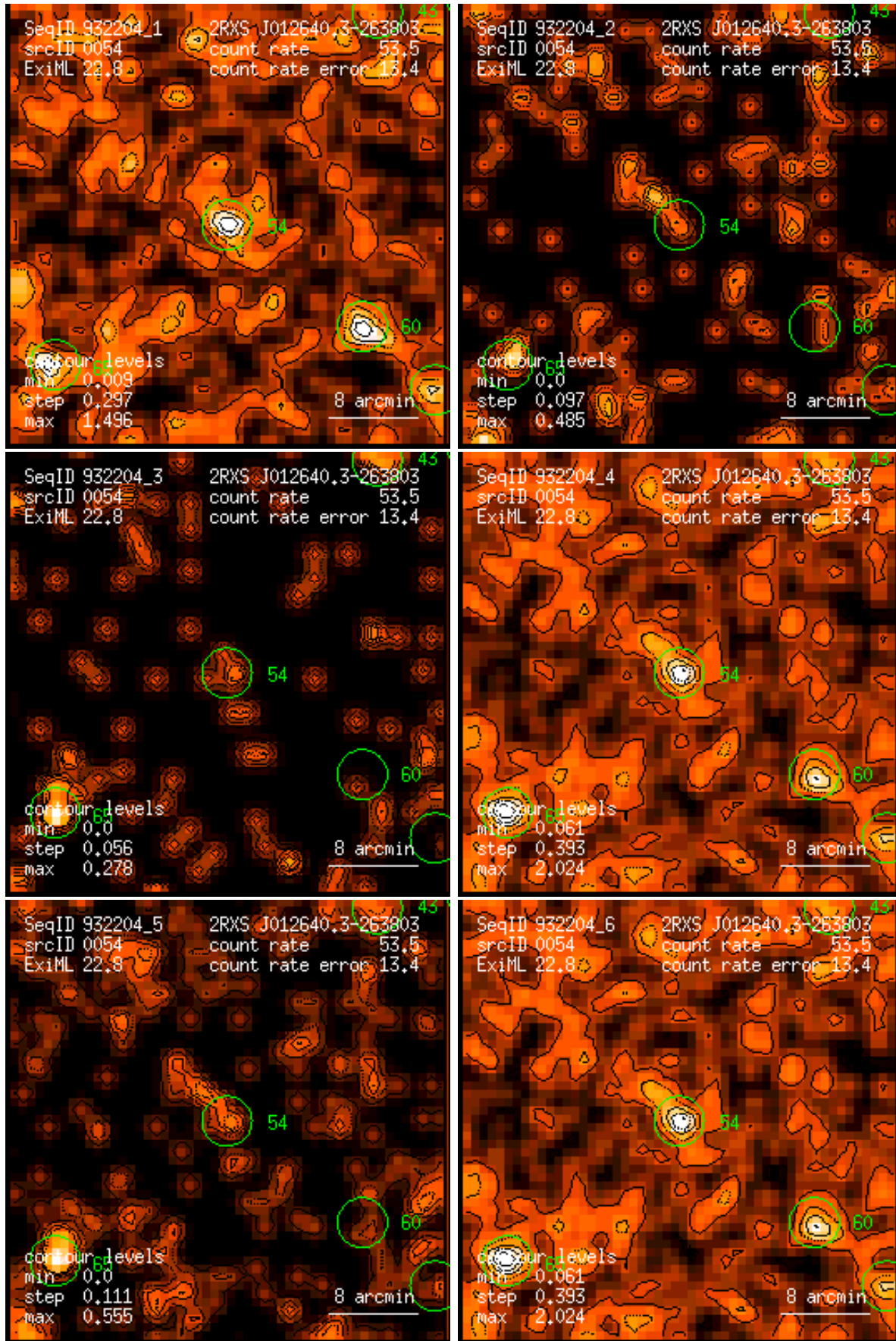
Figure 54: RASS 932204: detection 0054: band rate images, Gaussian filter: (1) PSPC channels 11 – 41, (2) 52 – 90, (3) 91 – 201, (4) 11 – 235, (5) 52 – 201, (6) 11 – 201. Broad band rates in counts/ks. Band rate contour levels in counts/ks/arcmin 2 .
