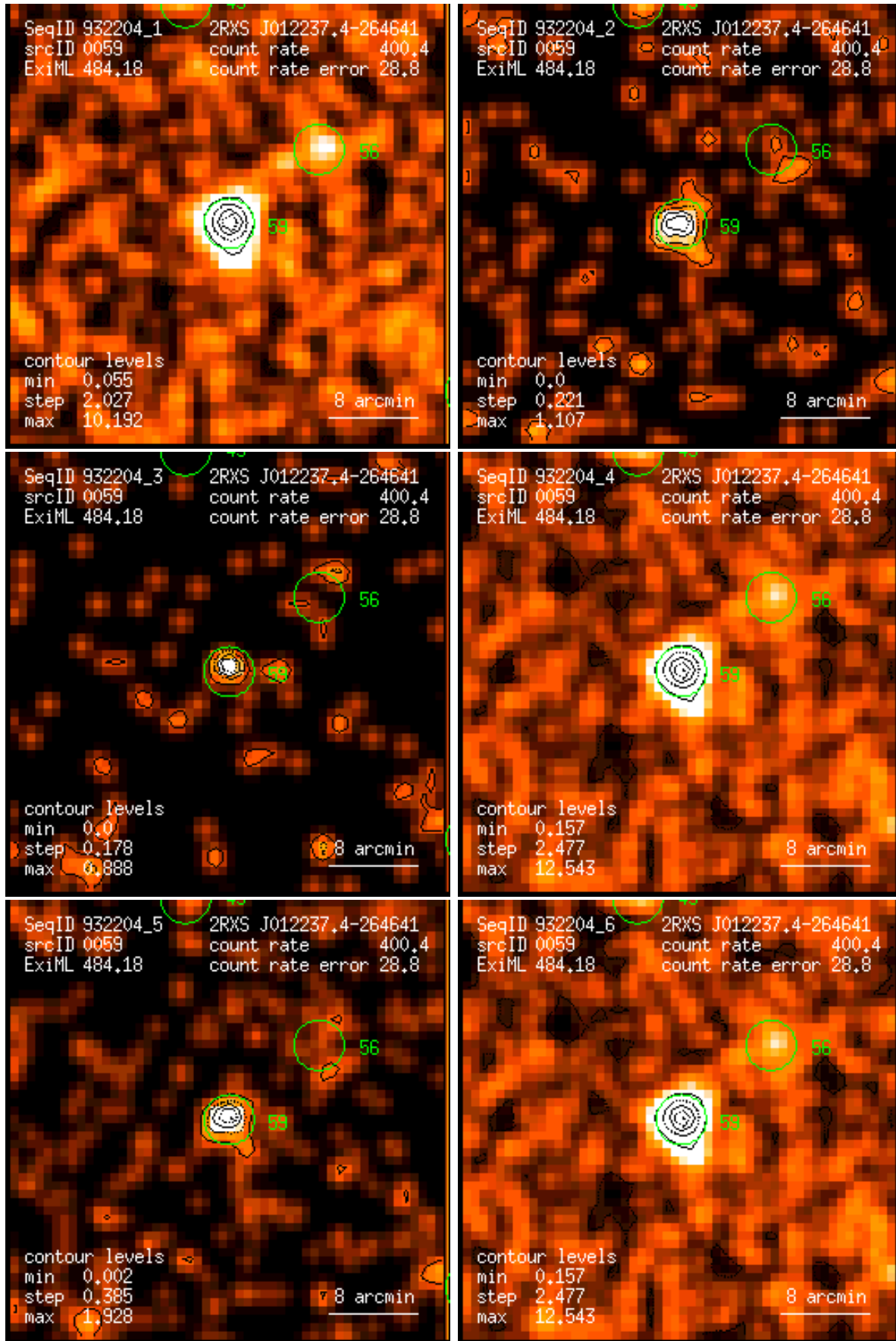
Figure 59: RASS 932204: detection 0059: band rate images, Gaussian filter: (1) PSPC channels 11 – 41, (2) 52 – 90, (3) 91 – 201, (4) 11 – 235, (5) 52 – 201, (6) 11 – 201. Broad band rates in counts/ks. Band rate contour levels in counts/ks/arcmin 2 .
