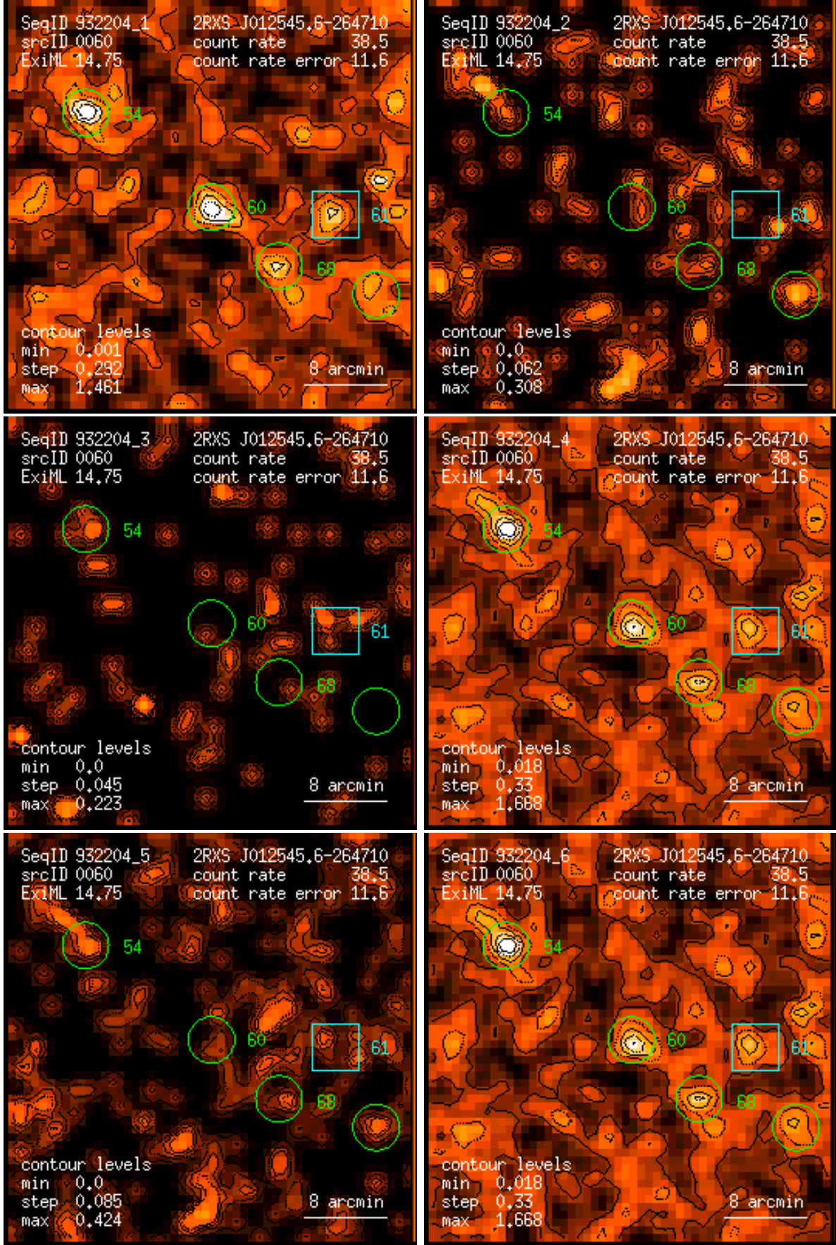
Figure 60: RASS 932204: detection 0060: band rate images, Gaussian filter: (1) PSPC channels 11 – 41, (2) 52 – 90, (3) 91 – 201, (4) 11 – 235, (5) 52 – 201, (6) 11 – 201. Broad band rates in counts/ks. Band rate contour levels in counts/ks/arcmin 2 .
