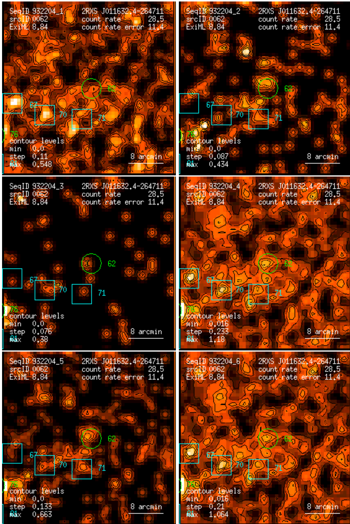
Figure 62: RASS 932204: detection 0062: band rate images, Gaussian filter: (1) PSPC channels 11 – 41, (2) 52 – 90, (3) 91 – 201, (4) 11 – 235, (5) 52 – 201, (6) 11 – 201. Broad band rates in counts/ks. Band rate contour levels in counts/ks/arcmin 2 .
