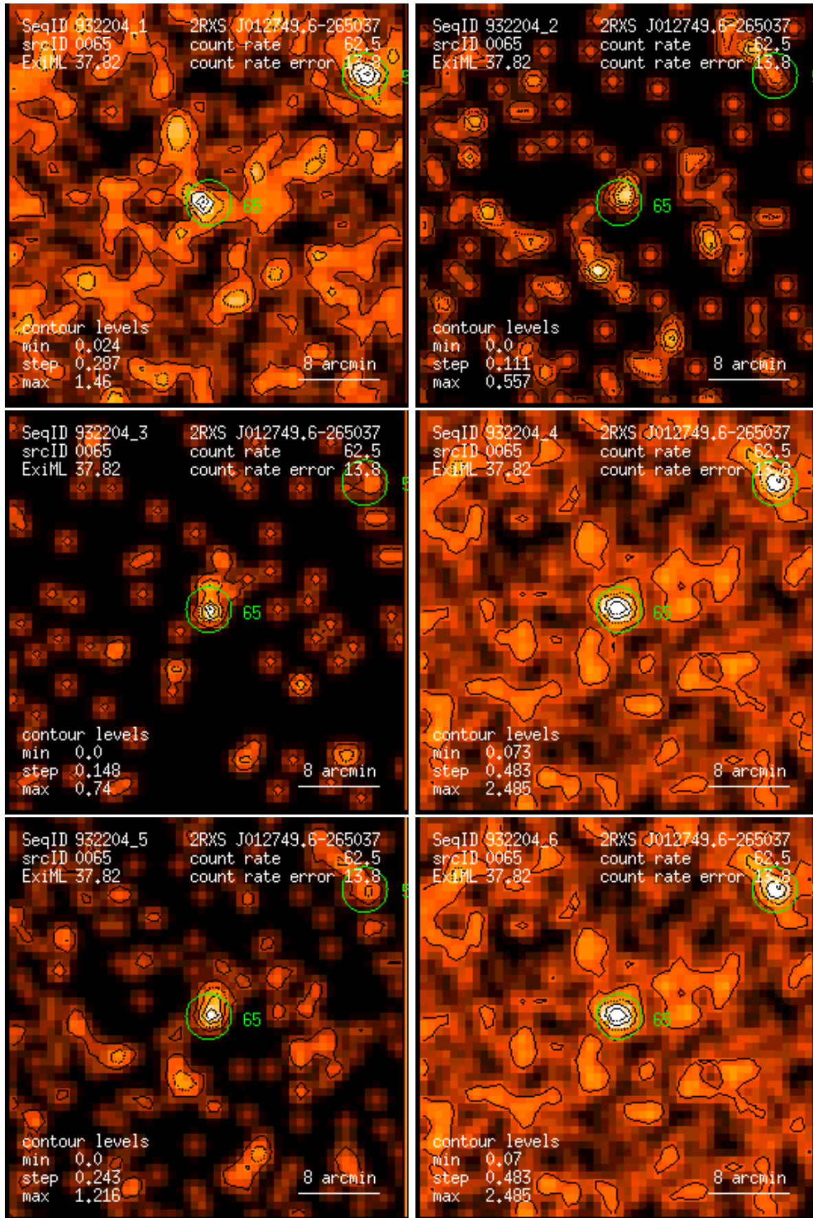
Figure 65: RASS 932204: detection 0065: band rate images, Gaussian filter: (1) PSPC channels 11 – 41, (2) 52 – 90, (3) 91 – 201, (4) 11 – 235, (5) 52 – 201, (6) 11 – 201. Broad band rates in counts/ks. Band rate contour levels in counts/ks/arcmin 2 .
