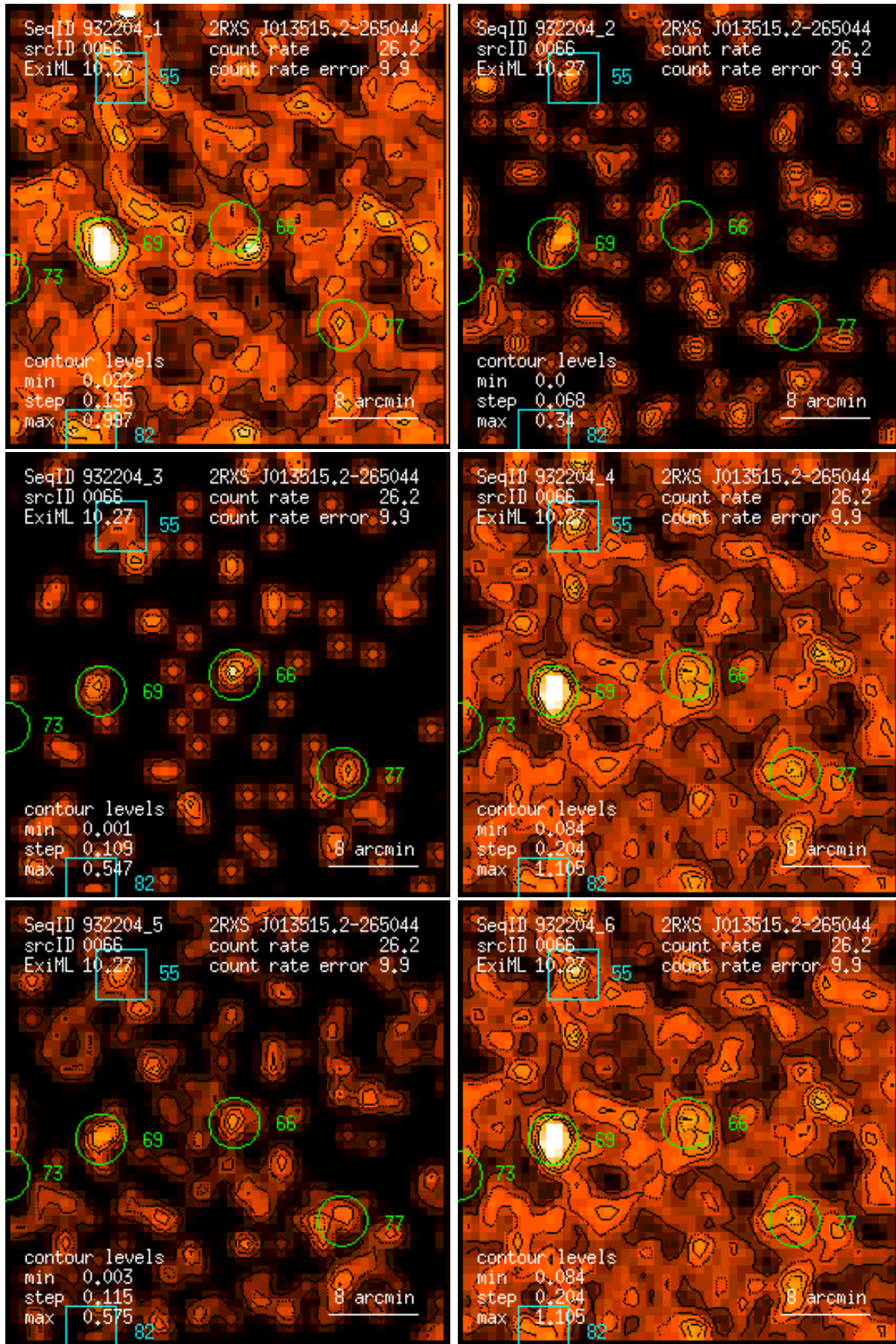
Figure 66: RASS 932204: detection 0066: band rate images, Gaussian filter: (1) PSPC channels 11 – 41, (2) 52 – 90, (3) 91 – 201, (4) 11 – 235, (5) 52 – 201, (6) 11 – 201. Broad band rates in counts/ks. Band rate contour levels in counts/ks/arcmin 2 .
