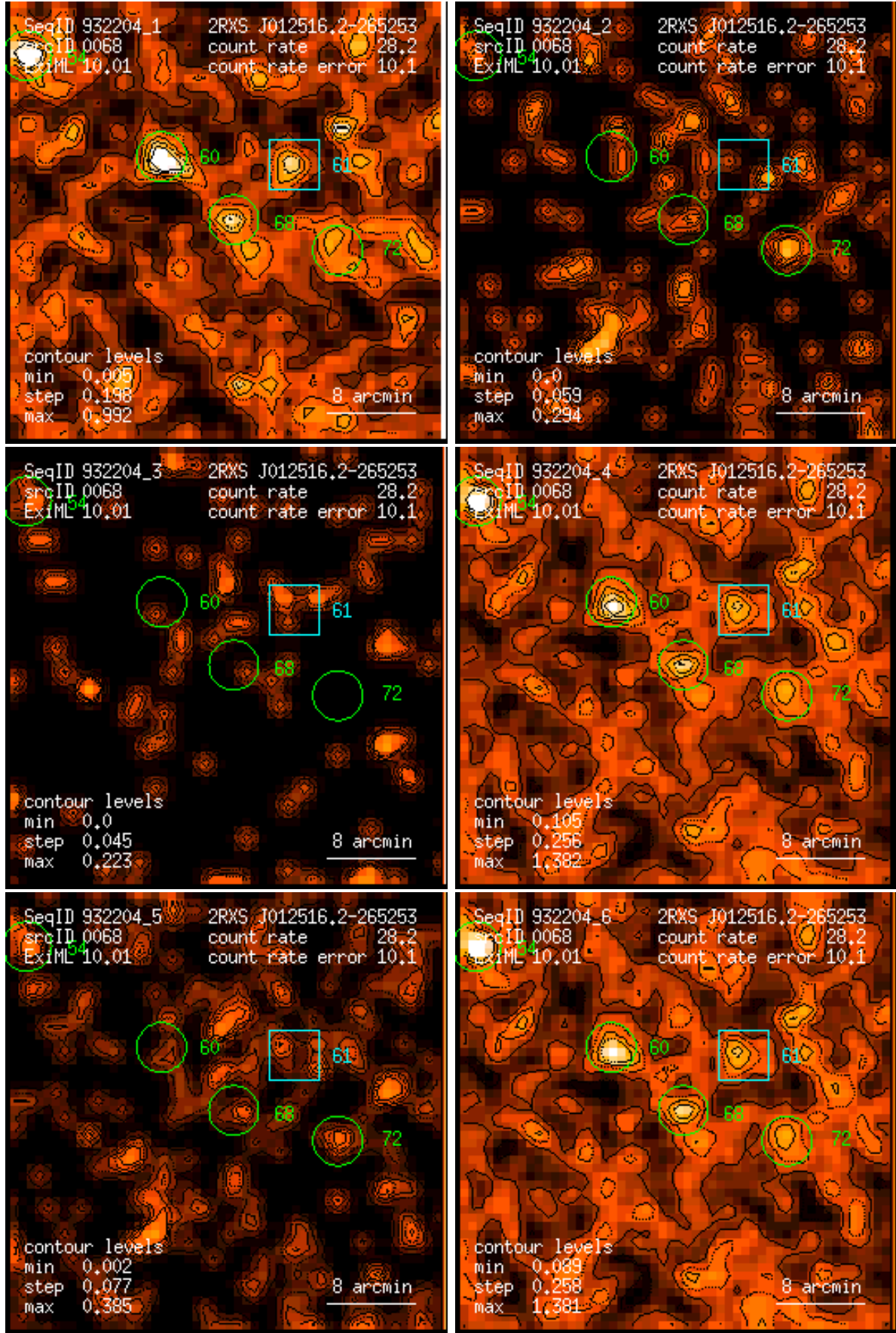
Figure 68: RASS 932204: detection 0068: band rate images, Gaussian filter: (1) PSPC channels 11 – 41, (2) 52 – 90, (3) 91 – 201, (4) 11 – 235, (5) 52 – 201, (6) 11 – 201. Broad band rates in counts/ks. Band rate contour levels in counts/ks/arcmin 2 .
