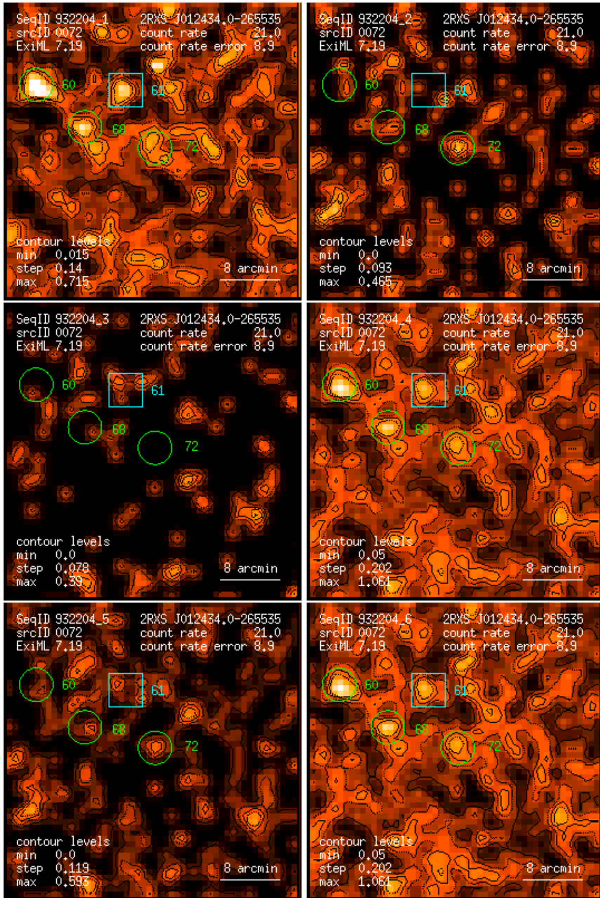
Figure 72: RASS 932204: detection 0072: band rate images, Gaussian filter: (1) PSPC channels 11 – 41, (2) 52 – 90, (3) 91 – 201, (4) 11 – 235, (5) 52 – 201, (6) 11 – 201. Broad band rates in counts/ks. Band rate contour levels in counts/ks/arcmin 2 .
