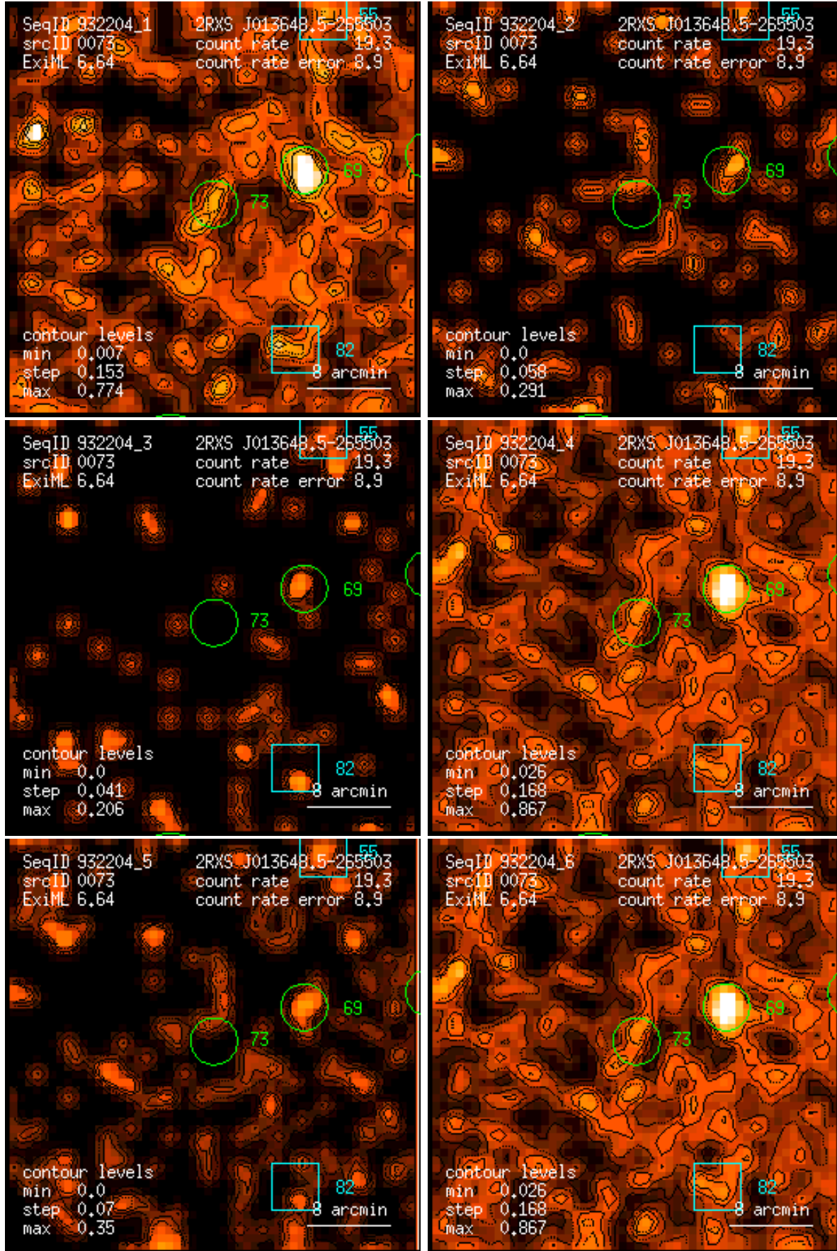
Figure 73: RASS 932204: detection 0073: band rate images, Gaussian filter: (1) PSPC channels 11 – 41, (2) 52 – 90, (3) 91 – 201, (4) 11 – 235, (5) 52 – 201, (6) 11 – 201. Broad band rates in counts/ks. Band rate contour levels in counts/ks/arcmin 2 .
