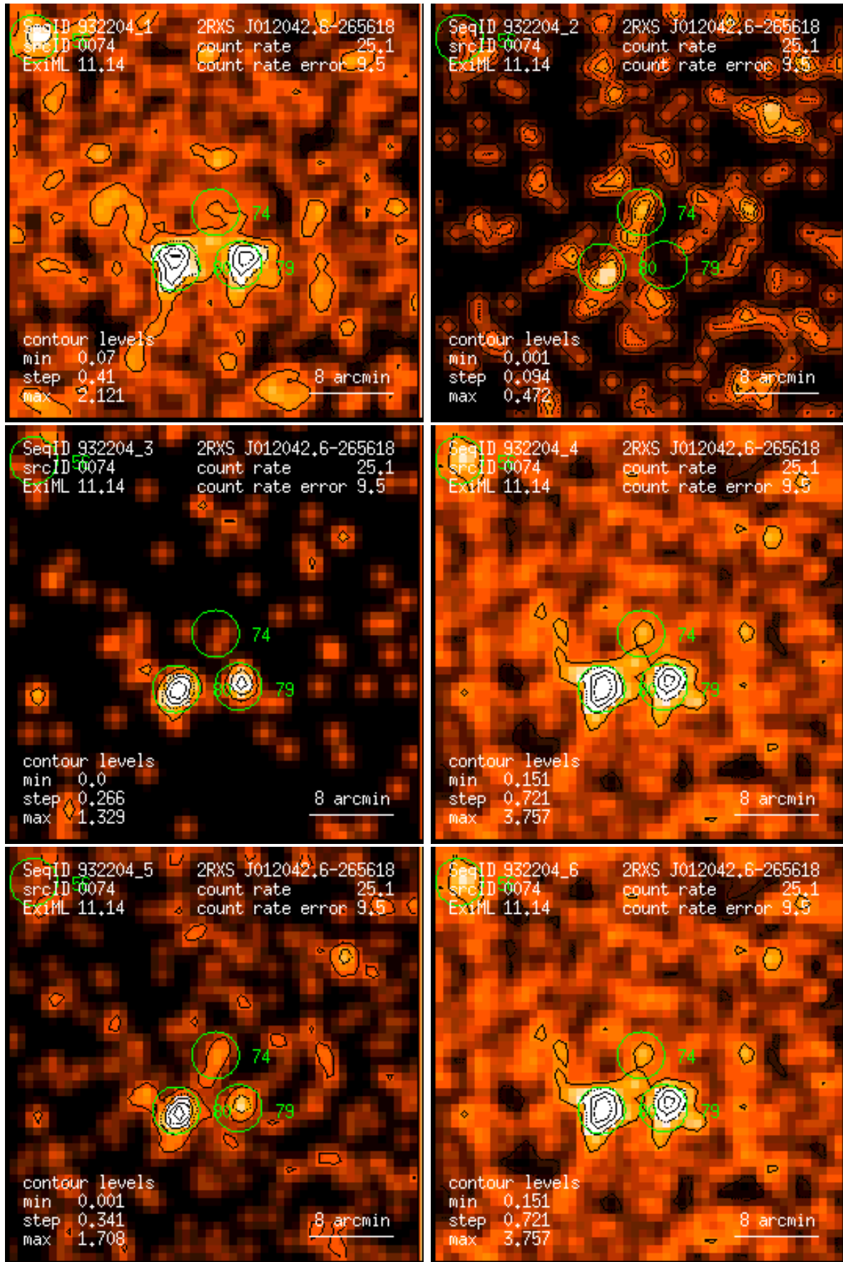
Figure 74: RASS 932204: detection 0074: band rate images, Gaussian filter: (1) PSPC channels 11 – 41, (2) 52 – 90, (3) 91 – 201, (4) 11 – 235, (5) 52 – 201, (6) 11 – 201. Broad band rates in counts/ks. Band rate contour levels in counts/ks/arcmin 2 .
