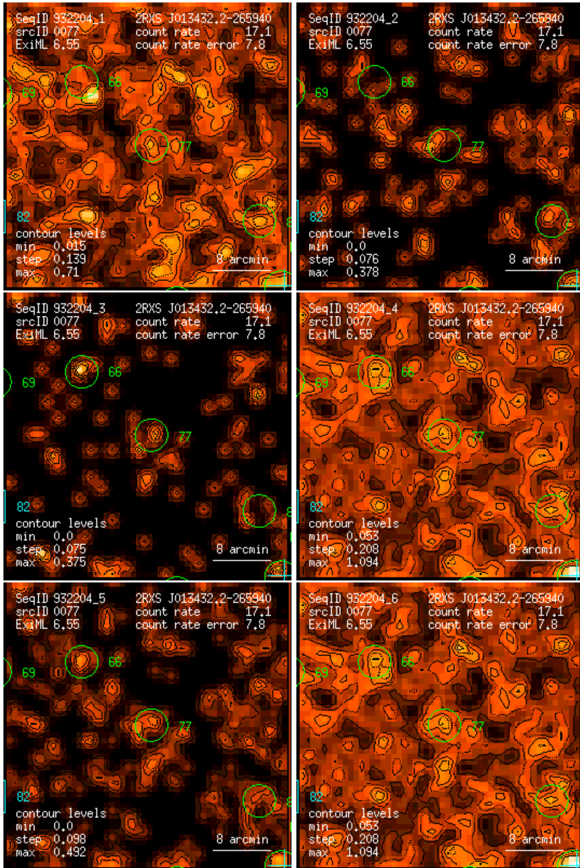
Figure 77: RASS 932204: detection 0077: band rate images, Gaussian filter: (1) PSPC channels 11 – 41, (2) 52 – 90, (3) 91 – 201, (4) 11 – 235, (5) 52 – 201, (6) 11 – 201. Broad band rates in counts/ks. Band rate contour levels in counts/ks/arcmin 2 .
