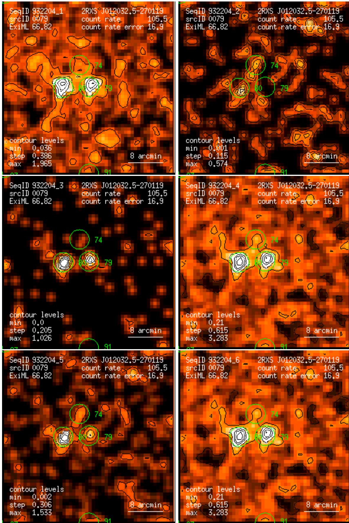
Figure 79: RASS 932204: detection 0079: band rate images, Gaussian filter: (1) PSPC channels 11 – 41, (2) 52 – 90, (3) 91 – 201, (4) 11 – 235, (5) 52 – 201, (6) 11 – 201. Broad band rates in counts/ks. Band rate contour levels in counts/ks/arcmin 2 .
