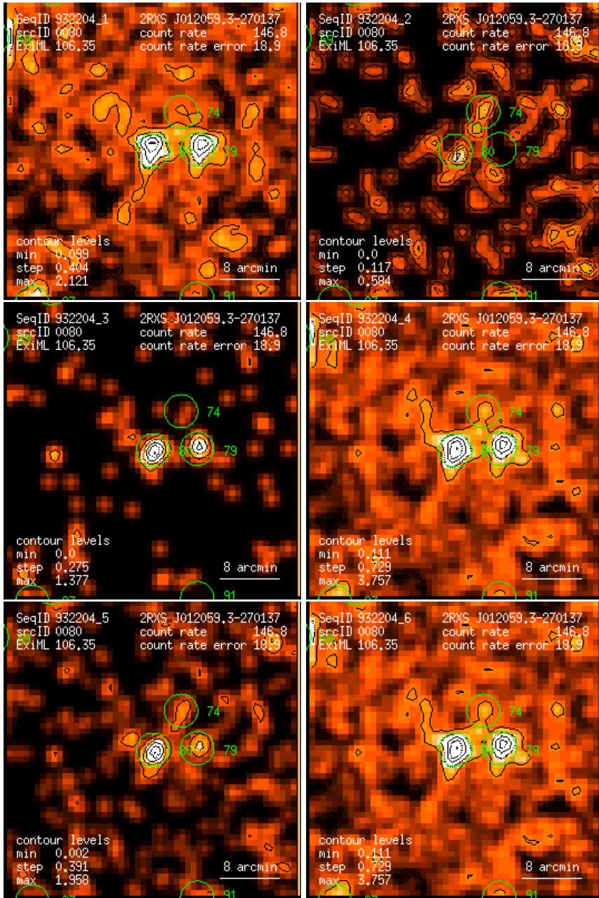
Figure 80: RASS 932204: detection 0080: band rate images, Gaussian filter: (1) PSPC channels 11 – 41, (2) 52 – 90, (3) 91 – 201, (4) 11 – 235, (5) 52 – 201, (6) 11 – 201. Broad band rates in counts/ks. Band rate contour levels in counts/ks/arcmin 2 .
