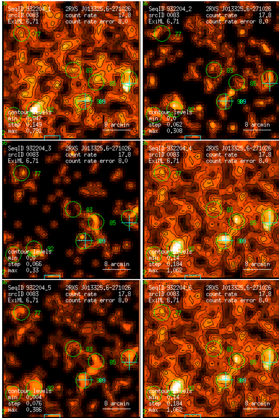
Figure 83: RASS 932204: detection 0083: band rate images, Gaussian filter: (1) PSPC channels 11 – 41, (2) 52 – 90, (3) 91 – 201, (4) 11 – 235, (5) 52 – 201, (6) 11 – 201. Broad band rates in counts/ks. Band rate contour levels in counts/ks/arcmin 2 .
