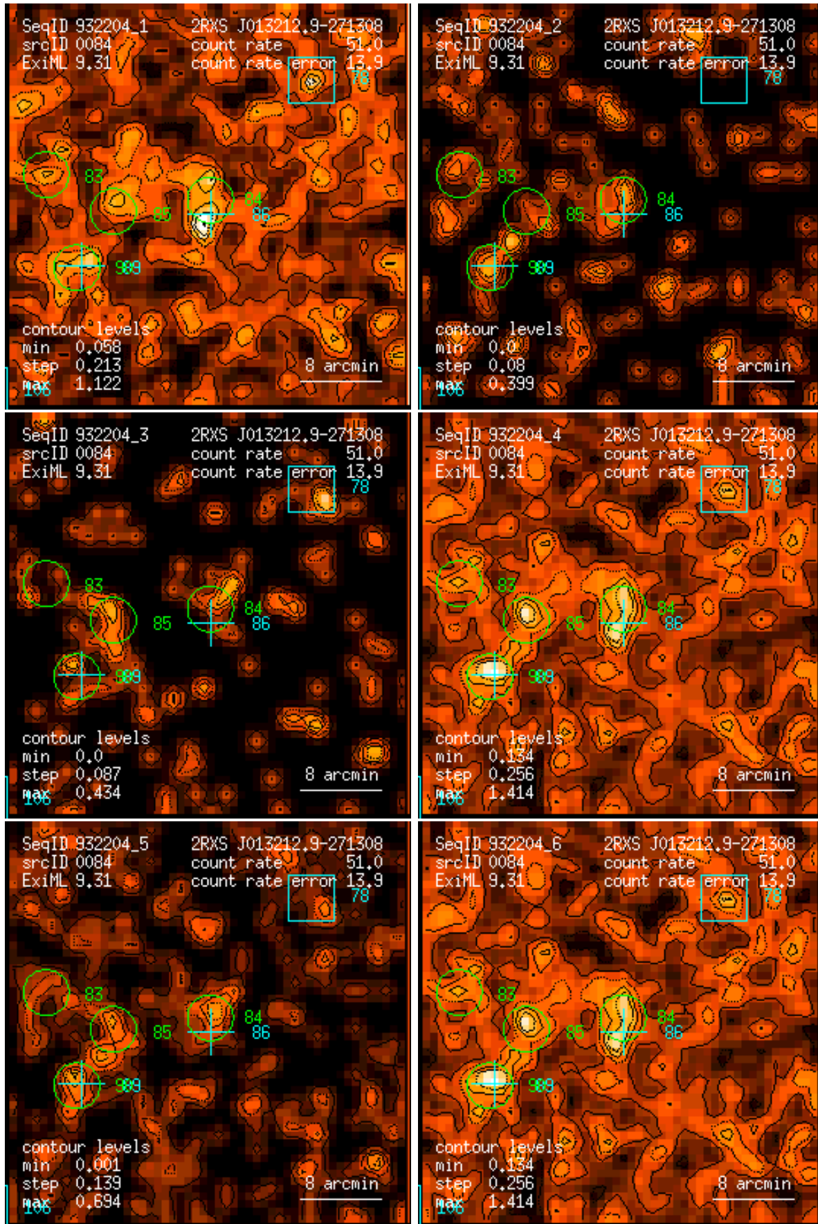
Figure 84: RASS 932204: detection 0084: band rate images, Gaussian filter: (1) PSPC channels 11 – 41, (2) 52 – 90, (3) 91 – 201, (4) 11 – 235, (5) 52 – 201, (6) 11 – 201. Broad band rates in counts/ks. Band rate contour levels in counts/ks/arcmin 2 .
