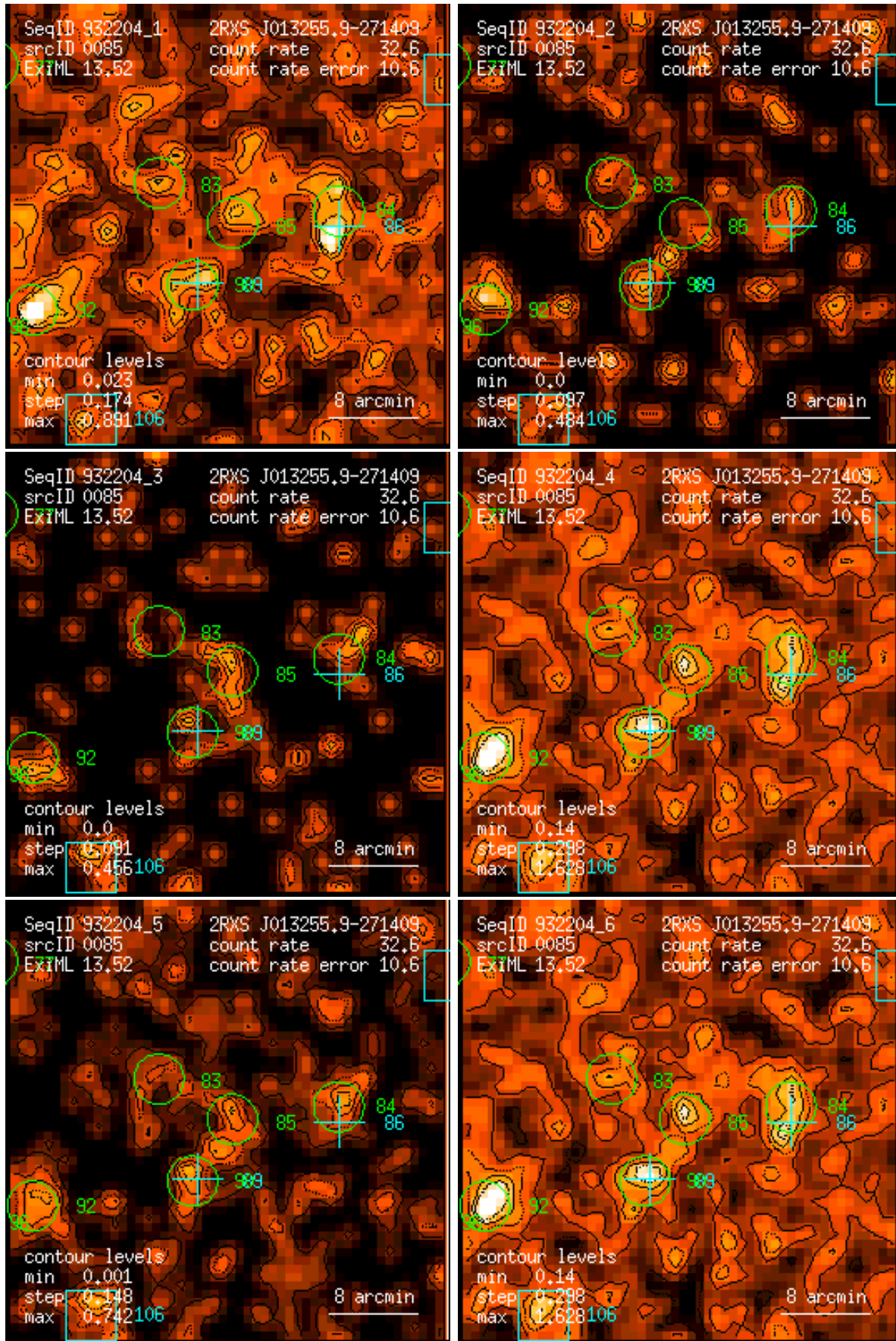
Figure 85: RASS 932204: detection 0085: band rate images, Gaussian filter: (1) PSPC channels 11 – 41, (2) 52 – 90, (3) 91 – 201, (4) 11 – 235, (5) 52 – 201, (6) 11 – 201. Broad band rates in counts/ks. Band rate contour levels in counts/ks/arcmin 2 .
