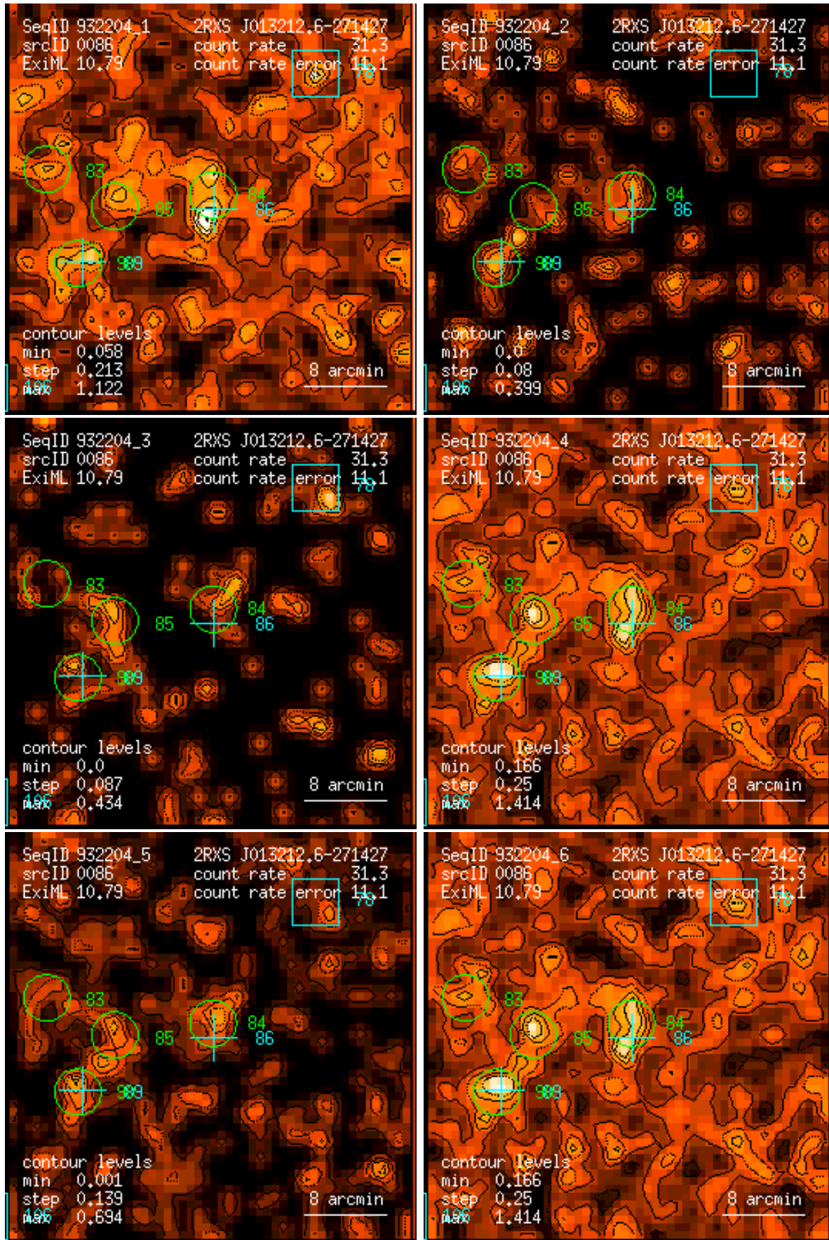
Figure 86: RASS 932204: detection 0086: band rate images, Gaussian filter: (1) PSPC channels 11 – 41, (2) 52 – 90, (3) 91 – 201, (4) 11 – 235, (5) 52 – 201, (6) 11 – 201. Broad band rates in counts/ks. Band rate contour levels in counts/ks/arcmin 2 .
