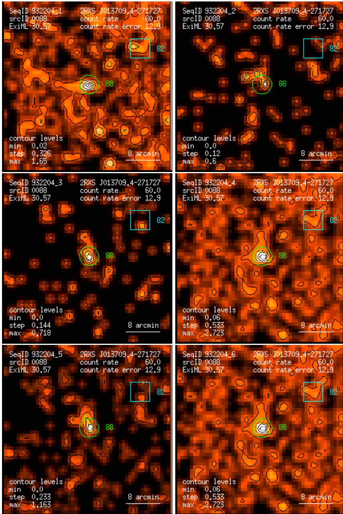
Figure 88: RASS 932204: detection 0088: band rate images, Gaussian filter: (1) PSPC channels 11 – 41, (2) 52 – 90, (3) 91 – 201, (4) 11 – 235, (5) 52 – 201, (6) 11 – 201. Broad band rates in counts/ks. Band rate contour levels in counts/ks/arcmin 2 .
